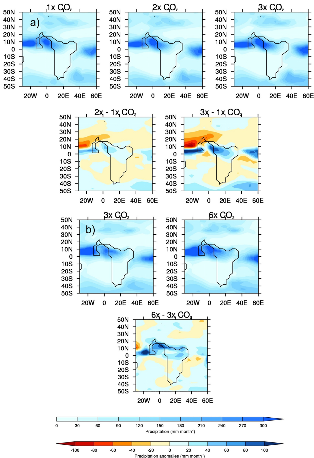
Figure 5. JJA precipitation multi-model ensemble mean (MME) climatology absolutes and anomalies for the 1x, 2x, 3x, and 6x CO 2 experiments, using both samples: (a) Lower-level sample of CO 2 experiments (comprising the four models that conducted these: GFDL_CM2.1, HadCM3B_M2.1aN, HadCM3BL_M2.1aN, and MIROC4m), absolutes (top row) and anomalies (second row); (b) Higher-level sample of CO 2 experiments (comprising the two models that conducted these: CESM1.2_CAM5 and GFDL_CM2.1), absolutes (top row) and anomalies (second row).
