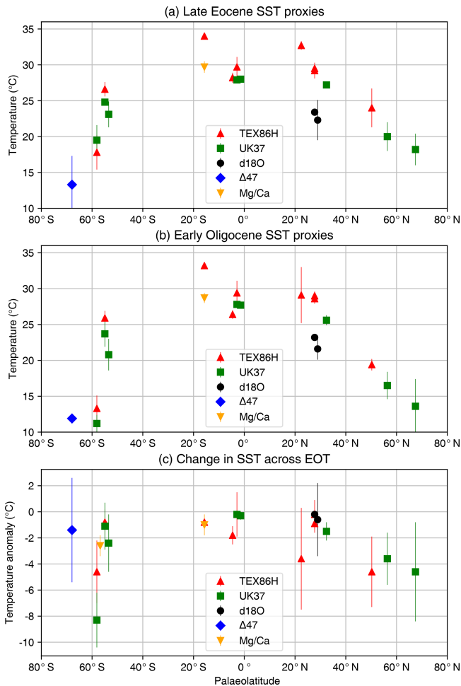
Figure 3. Summary of sea surface temperature (SST) change across the EOT from proxies \text{TEX}_{86}^H , U_{37}^{K'} , \delta^{18}\text{O} , \Delta_{47} , and Mg/Ca. (a) Late Eocene, (b) early Oligocene and (c) change in SST across the EOT. Data shown in panels (a) and (b) are only from locations that record a temperature signal on both sides of the EOT. Data compiled from Bohaty et al. (2012), Cramwinckel et al. (2018), Inglis et al. (2015), Kobashi et al. (2004), Lear et al. (2008), Liu et al. (2009, 2018), Pearson et al. (2007), Petersen and Schrag (2015), Piga (2020), Śliwińska et al. (2019), Wade et al. (2012) and Zhang et al. (2013). The late Eocene value was calculated as an average between 38 and 33.9 Ma (pre-EOT), while the early Oligocene value was calculated as the average between 33.9 and 30 Ma (post-EOT), and the change across the EOT is the difference between these values. The data compilation is provided in digital form in Table S1 in the Supplement.
