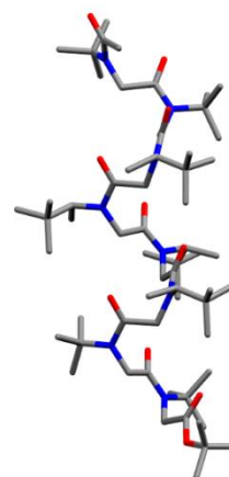
Fig.5. X-ray structure of octamer 19
