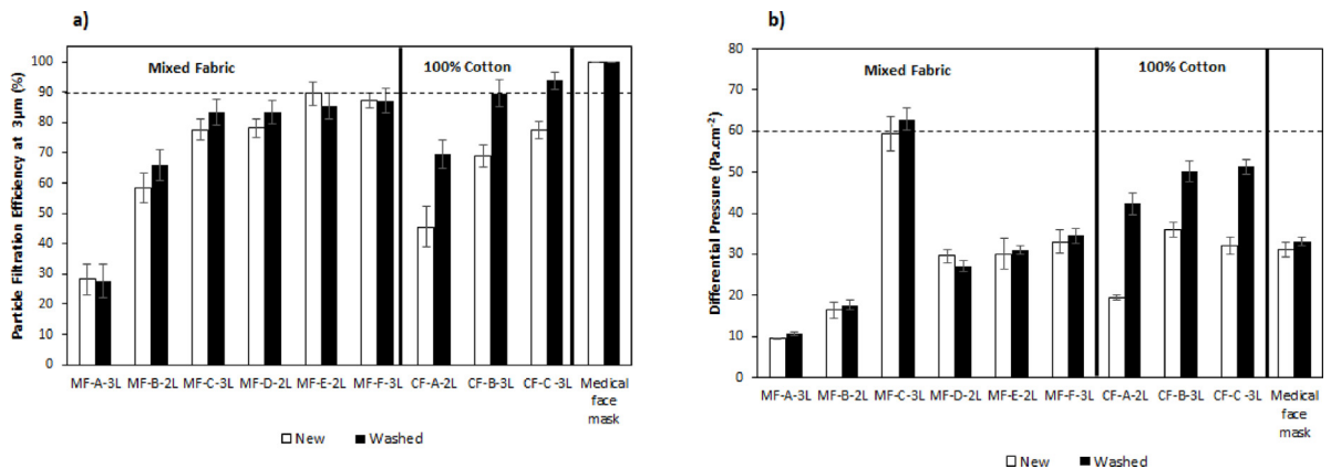
Fig. 6. Comparison of (a) particle filtration efficiency (%) for 3 μm particle sizes and (b) differential pressure (Pa cm -2 ) for the mixed fabric, 100% cotton and medical face masks. Average values (N = 3) ± standard-deviation for particle filtration efficiency and Average values (N = 5) ± standard-deviation for differential pressure. MF: Mixed Fabric, CF: Cotton Fabric, 2L: 2-Layer, 3L: 3-Layer.
