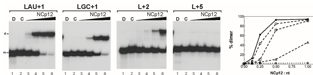
Figure 7. Influence of stem C extensions on NCp12-mediated L3 RNA dimerization. The 5'-end-labeled L RNAs in the absence (lanes C) or the presence of NCp12 (lanes 3–6) were incubated at 37 °C as described in Materials and Methods. After phenol–chloroform extraction, the samples were analyzed by electrophoresis on 12% polyacrylamide gels at 25 °C in the TBE buffer. Heat-denatured L RNAs (lanes D) were used to identify the bands corresponding to monomeric L RNAs. Lanes 3–6, protein to nucleotide molar ratios were 1:8, 1:4, 1:2, and 1:1. The monomeric and dimeric forms of L RNAs are indicated by m and d, respectively. The graph was derived from the gels shown in this figure and Figure 4. Filled circles, Lwt RNA; open circles, LAU+1 RNA; open squares, LGC+1 RNA; open triangles, L+2 RNA; open diamonds, L+5 RNA.
