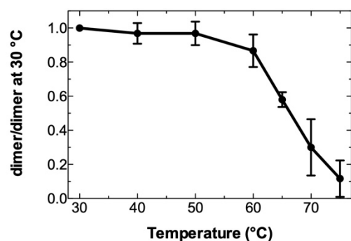
Figure 5. Thermal stability of the dimeric LdLB RNA. The melting curve was determined as described in Materials and Methods. Data are normalized according to the percentage of dimer at 30 °C and result from three experiments. Error bars show standard deviations.
