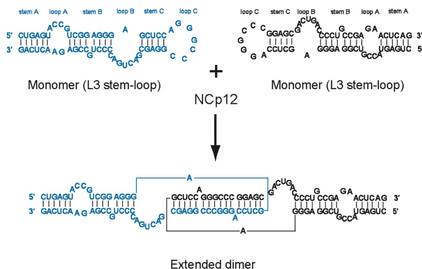
Figure 2. Secondary structures for the L3 stem-loop in the monomer and the extended dimer.
