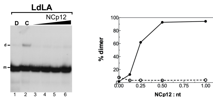
Figure 6. Deletion of loop A and the G bulge prevents NCp12-mediated L3 RNA dimerization. The 5'-end-labeled LdLA RNA in the absence (lane C) or the presence of NCp12 (lanes 3–6) was incubated at 37 °C as described in Materials and Methods. After phenol–chloroform extraction, the samples were analyzed by electrophoresis on a 12% polyacrylamide gel at 25 °C in the TBE buffer. Heat-denatured LdLA RNA (lane D) was used to identify the band corresponding to monomeric LdLA RNA. Lanes 3–6, protein to nucleotide molar ratios were 1:8, 1:4, 1:2, and 1:1. The monomeric and dimeric forms of LdLA RNA are indicated by m and d, respectively. The graph was derived from the gels shown in this figure and Figure 4. Filled circles, Lwt; open circles, LdLA.
