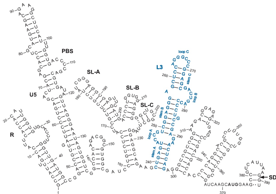
Figure 1. Predicted secondary structures for the ALV 5'-leader RNA [30]. Numbering is relative to the genomic RNA cap site (+1). R, repeated sequence; U5, unique sequence in 5'; PBS, primer binding site; SL-A, B, and C, stem-loop structures of the minimal packaging signal [31]; L3 in blue font, stem-loop structure involved in ALV gRNA dimerization; the structural elements of L3 are indicated in blue; AUG in bold, gag initiation codon; SD, splice donor site.
