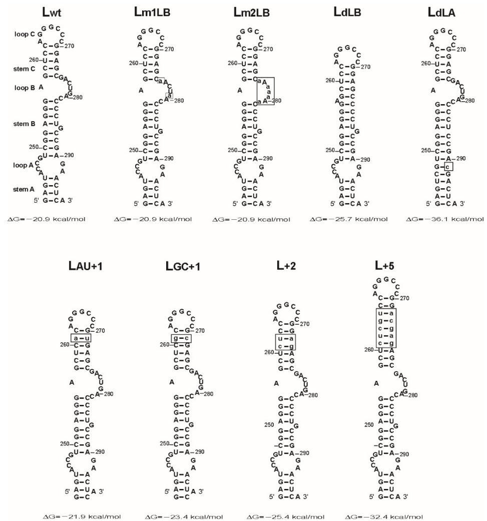
Figure 3. Predicted secondary structures for the L3 sequence of LRNAs containing mutations or deletions. The mfold program [40] predicted the most stable secondary structure for each RNA. Numbering is relative to the genomic RNA cap site (+1). The lower-case letters in the boxes indicate the mutations.
