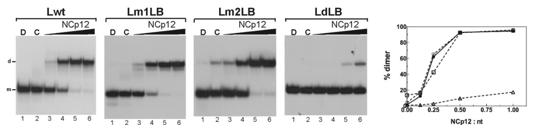
Figure 4. Dimerization of L RNAs harboring mutations in loop B. The 5'-end-labeled L RNAs in the absence (lanes C) or the presence of NCp12 (lanes 3–6) were incubated at 37 °C as described in Materials and Methods. After phenol–chloroform extraction, the samples were analyzed by electrophoresis on 12% polyacrylamide gels at 25 °C in the TBE buffer. Heat-denatured L RNAs (lanes D) were used to identify the bands corresponding to monomeric L RNAs. Lanes 3–6, protein to nucleotide molar ratios were 1:8, 1:4, 1:2, and 1:1. The monomeric and dimeric forms of L RNAs are indicated by m and d, respectively. The graph was derived from the gels shown in this figure. Filled circles, Lwt RNA; open circles, Lm1LB RNA; open squares, Lm2LB RNA; open triangles, LdLB RNA.
