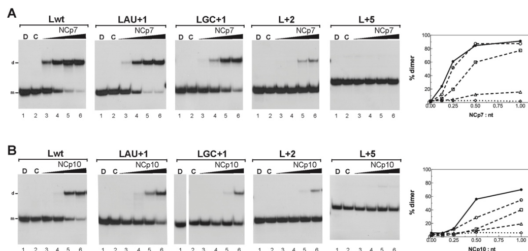
Figure 8. Influence of stem C extensions on L3 RNA dimerization induced by NCp7 and NCp10. (A) NCp7-mediated L3 RNA dimerization. (B) NCp10-mediated L3 RNA dimerization. The 5′-end-labeled L RNAs in the absence (lanes C) or the presence of NCp7 or NCp10 (lanes 3–6) were incubated at 37 °C as described in Materials and Methods. After phenol–chloroform extraction, the samples were analyzed by electrophoresis on 12% polyacrylamide gels at 25 °C in the TBE buffer. Heat-denatured L RNAs (lanes D) were used to identify the bands corresponding to monomeric L RNAs. Lanes 3–6, protein to nucleotide molar ratios were 1:8, 1:4, 1:2, and 1:1. The monomeric and dimeric forms of L RNAs are indicated by m and d, respectively. The graphs were derived from the gels shown in this figure. Filled circles, Lwt RNA; open circles, LAU+1 RNA; open squares, LGC+1 RNA; open triangles, L+2 RNA; open diamonds, L+5 RNA.
