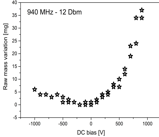
Figure 9: Effect of the high voltage DC bias on the mass variations, while the RF field is kept on at the frequency and power indicated in the inset. Here the device is oriented as in Fig. 2. The voltage has been varied from -1 KVolt to 1 KVolt and backwards, with steps of 100 Volts. The indication of raw mass variation is referred to the fact that data is untreated to compensate any eventual drift.
