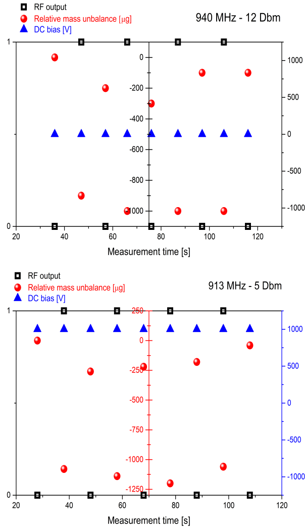
Figure 8: Outcomes relative to two typical experiments performed while applying the RF field and a DC bias. The RF source is switched on and off periodically, approximately every 10 seconds of acquisition (black open squares: '1' represents the device on, '0' represents the device off), at the frequency and power indicated in the top right inset. The DC bias is set at a fixed value (blue triangles). The balance readings are converted into a relative variation scale by taking as zero the initial value (red circles), and eventually removing the small linear drift that sometimes can be found, presumably due to heating/cooling phenomena during the day. The measure at 940 MHz was performed orienting the EMT as shown in Fig. 2, while the one at 913 MHz was performed by reversing the orientation.
