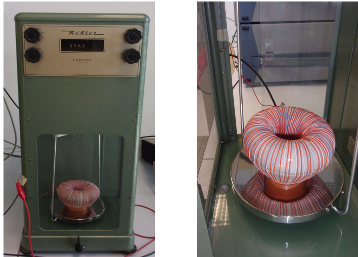
Figure 7: The device on the plate of the balance machine.
