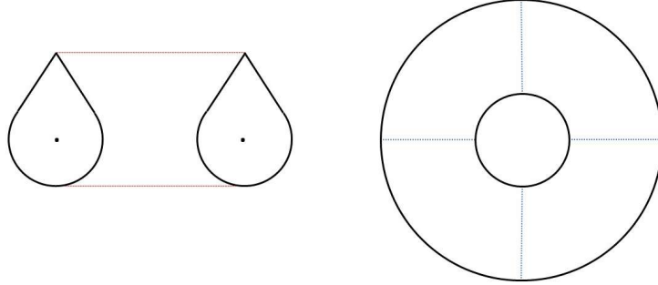
Figure 2: Possible configuration of a ring with asymmetric section (left: section view; right: top view).
