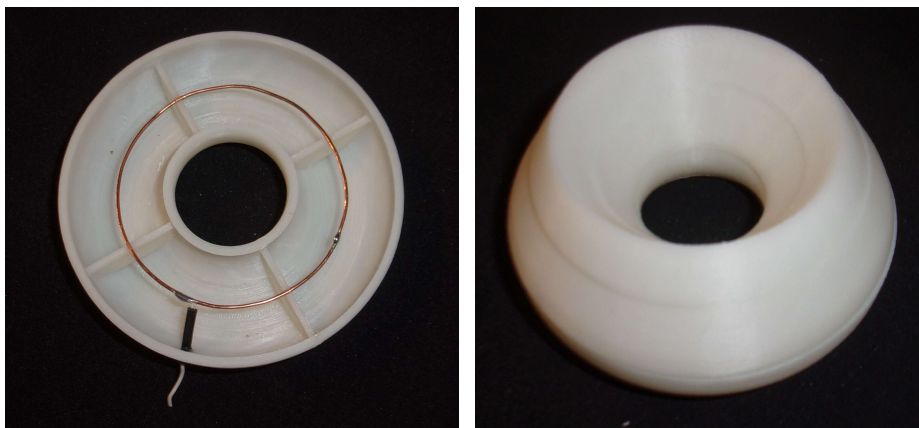
Figure 4: Printed support of the ring (left), relative to the bottom part. The internal copper loop, to be connected to ground through a small radial conductor, is visible. On the right, we can see the two parts assembled.
