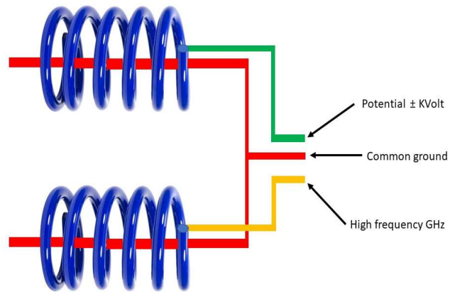
Figure 5: Electric scheme
