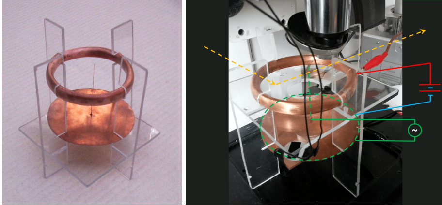
Figure 11: Left: the device tested in 2014. Right: device under test and labelling to describe how the measurement was conducted. The acrylic transparent structure is used to keep in position the ring and the RF antenna on the one side, and to provide a stable horizontal surface where the cantilever is positioned, to explore the pressure effects. The yellow arrows represent the laser beam directed to the cantilever and reflected towards the four quadrant photodetector. Red and blue lines represent the high voltage connection scheme (the ring on the one side, the copper dish on the other), while green lines represent the RF connection scheme (the central copper wire and the dish). A chip with silicon cantilever was positioned in correspondence with the point of reflection of the laser beam, centered using the microscope objective seen on top of the picture.
