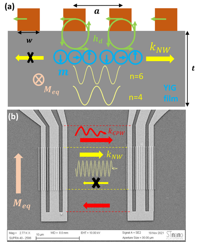
FIG. 1. (a) Sketch of the NWA-FMR mediated chiral coupling mechanism. (b) SEM image of device I, w = 300 nm width and a = 500 nm lattice constant of Ni 80 Fe 20 NWA grown on top of 55 nm thick YIG film, 80 nm Au-antennas grown on top of YIG|Ni 80 Fe 20 . Red and Yellow color represent respectively antenna ( k_{CPW} ) and Ni 80 Fe 20 NWA ( k_{NW} ) excite mode.
