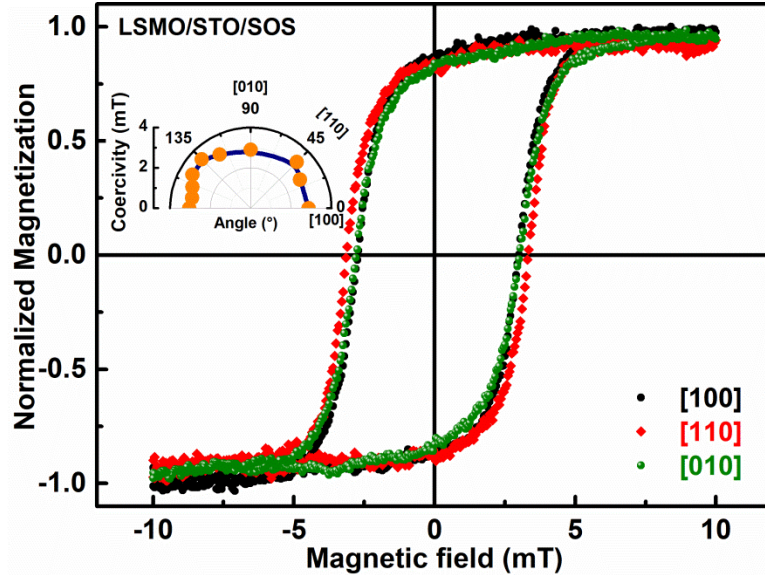
Figure 4: Room temperature angular-dependent in-plane MOKE hysteresis loops of LSMO film deposited on STO buffered SOS substrate. Inset shows its angular-dependent coercivity.
