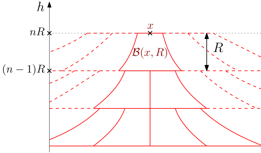
Figure 13: Box-tiling
