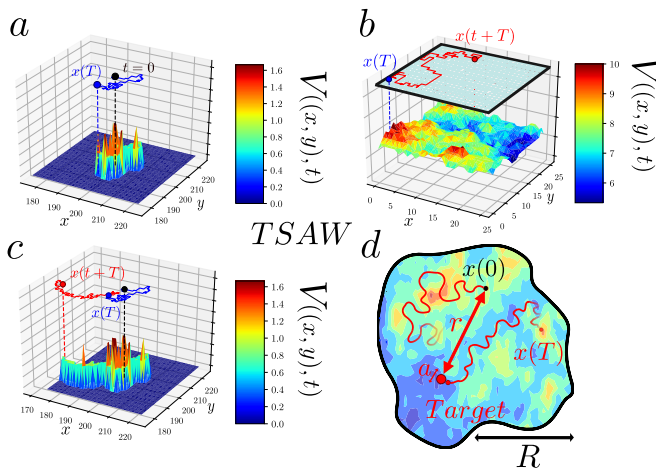
Figure 1. Aging and first-passage times for self-interacting random walks in infinite space and in confined domains. Examples of 2d self-interacting trajectories (TSAW model, see text) a . The random path from t = 0 to T generates the local energy landscape V((x, y), t) (proportional to the total number of visits to (x, y) until t ), plotted along the vertical axis z . This dynamics can lead to long range memory effects and aging at all time scales : the trajectory after T plotted in c , explicitly depends on the full territory visited by the walker until T . In confined domains b ., the statistics of visits to a given site is radically modified by confinement : the dynamics of self-interacting random walks is thus geometry dependent. d . In this article, we aim at quantifying space exploration and search kinetics of confined self-interacting random walks.
