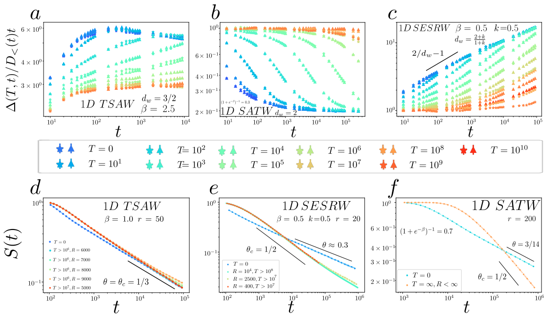
Figure 3. aging and first-passage properties for compact self-interacting random walks in infinite space and in confined geometries. aging of the increments for the 1d TSAW (a.), the 1d SATW (b.) and the 1d SESRW (c.) in both infinite space and confined domains (increments are normalized by the expected scaling for T \gg t ). The dynamic is found to be identical in infinite space (triangle) and in confined domains (stars) in both regimes t, T \ll R^{d_w} and T \gtrsim R^{d_w}, t \ll R^{d_w} . The TSAW is superdiffusive at all times scales and displays aging ; the SATW is diffusive at all times scales and displays aging. In contrast, the SESRW is diffusive for T \gg t , but superdiffusive for t \gg T with d_w = (2 + k)/(k + 1) . Persistence exponents in infinite space ( \theta ) and in confined domains ( \theta_c ) for the 1d TSAW (d.), the 1d SESRW (e.) and for the 1d SATW (f.). The persistence exponent is modified by confinement for the SATW and the SESRW models, but is found numerically to be unchanged for the TSAW.
