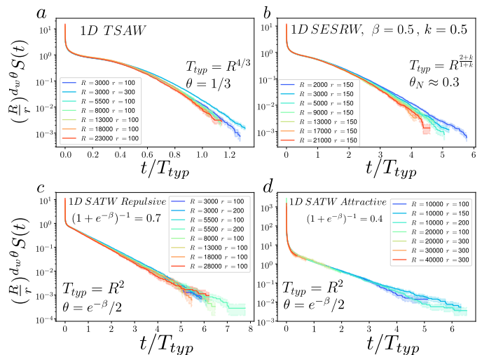
Figure 5. Asymptotic FPT distribution of compact self-interacting random walks in confined domains for fresh initial conditions. Here S(t) is the survival probability of the random walker, whose scaling with geometrical parameters is deduced from (21). The collapse of numerical simulations after rescaling for different values of geometric parameters captures the dependence of the FPT distribution on the geometric parameters r, R . Simulations are performed in 1D boxes of size R with reflecting boundary conditions. a. 1D TSAW with d_w = 3/2 (independent of \beta ). b. 1d SESRW with \beta = 0.5 and k = 0.5 . 1d repulsive SATW with (1 + e^{-\beta})^{-1} = 0.7 ( c. ) and (1 + e^{-\beta})^{-1} = 0.4 ( d. ).
