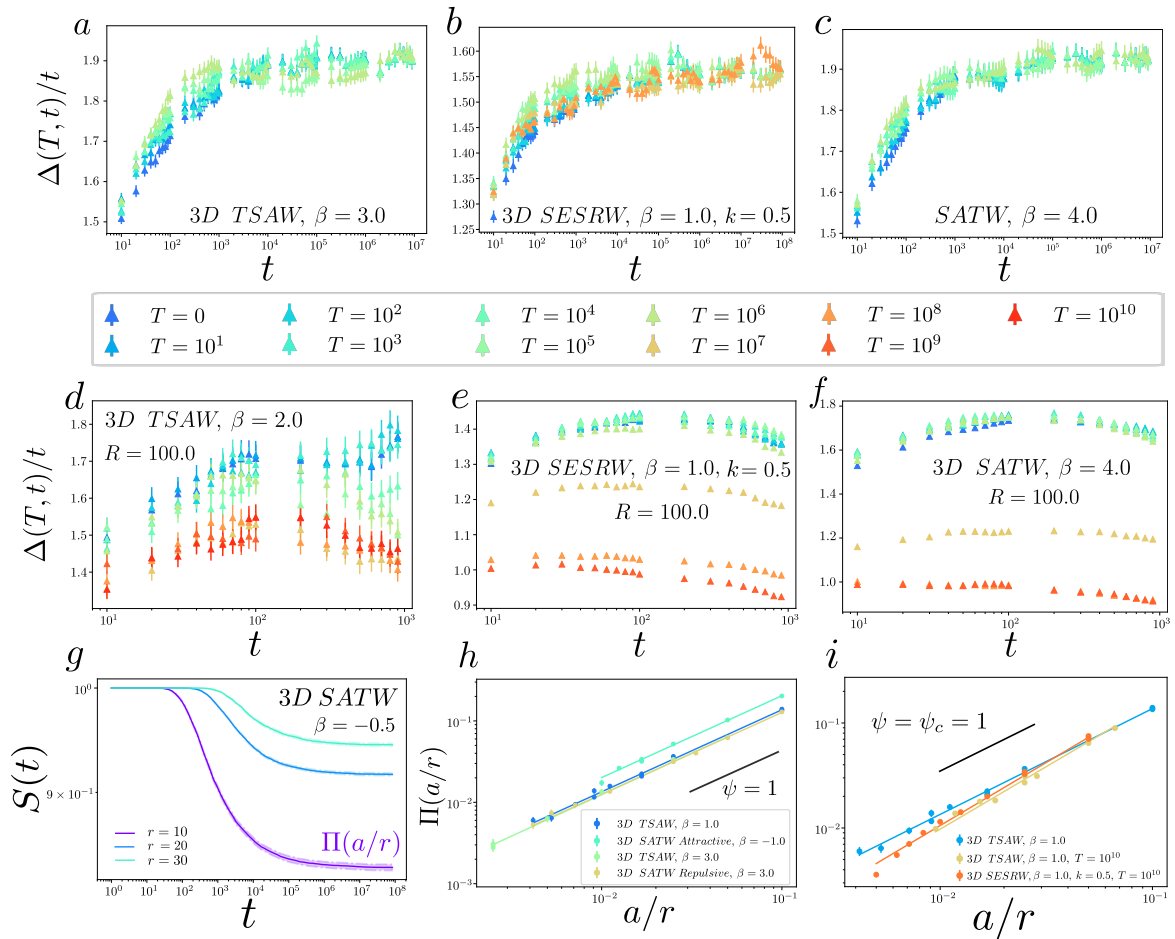
Figure 4. Aging and first-passage properties for non-compact self-interacting random walks in infinite space and in confined geometries. Aging of the increments for the 3d TSAW (a.), the 3d SESRW (b.) and the 3d SATW (c.) in infinite space (increments are normalized by the expected diffusive scaling at long times). Of note, the increments are stationary at timescales T \gg 1 . In contrast, in confined geometries, aging occurs at longer time scales \gtrsim R^d , for the TSAW (d.), the SESRW (e.) and the SATW (f.) (increments are normalized by the expected diffusive scaling at long times). g. For non-compact random walks (here the 3d diffusive SATW), the survival probability tends for t \rightarrow \infty to a non-zero value 1 - \Pi , which defines the hitting probability that depends on the initial distance to the target r and the target radius a . Hitting probability and transience exponent in infinite space (h.) and in confined domains (i.). Numerical simulations (symbols) and power law fits (plain lines). Our numerical results indicate \psi = \psi_c = 1 for the TSAW, the SESRW and the SATW, in agreement with the asymptotic diffusive behaviour of non compact self-interacting random walks.
