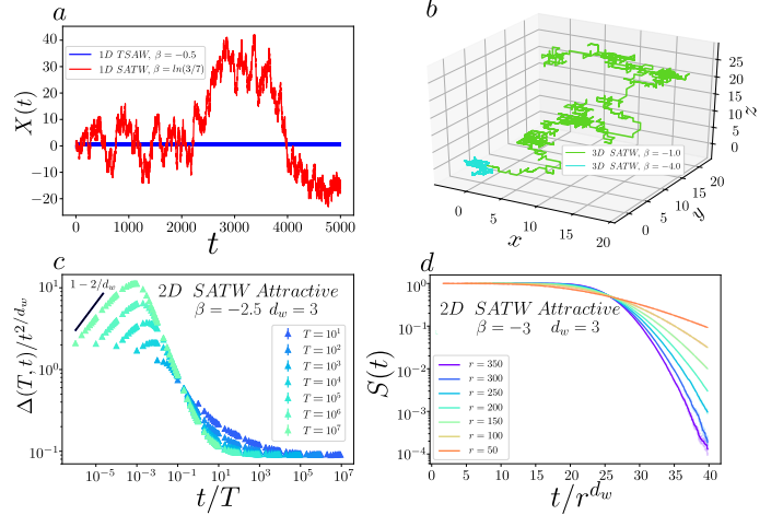
Figure 2. General properties of attractive self-interacting random walks. a. Example of trapped trajectory performed by a 1d attractive TSAW random walker (blue), compared to a diffusive trajectory of a 1d attractive SATW random walker (red). b. For d > 1 , the SATW is subdiffusive for |\beta| > |\beta_c| (blue sample trajectory), and diffusive for |\beta| < |\beta_c| (green sample trajectory). Here d = 3 and thus |\beta_c| \neq 0 [25]. c. Aging of the increments for the subdiffusive SATW ( d_w = 3 for d = 2 ) normalized by the expected subdiffusive scaling at long times. Each curve corresponds to a fixed value of T . Note that the increments are diffusive for t \ll T . d. In the subdiffusive regime, the SATW performs an extremely compact exploration of space : the survival probability S(t) decays faster than any powerlaw ( \theta = \infty ).
