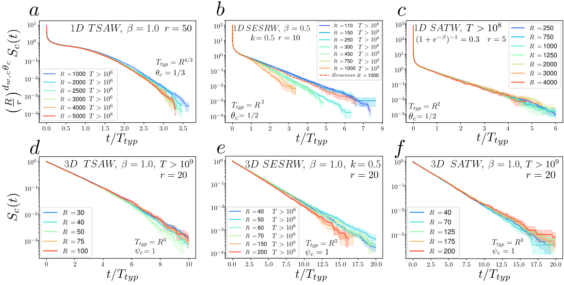
Figure 7. Asymptotic FPT distribution of self-interacting random walks in confined domains for aged initial conditions. The search process starts at t = 0 , but the random walker is assumed to have explored the domain from t = -T to t = 0 . S(t) is the survival probability of the random walker at time t . The scaling of S(t) with geometrical parameters is deduced from (30) and (32), for compact and non-compact processes respectively. The collapse of numerical simulations after rescaling captures the dependence of the FPT distribution on geometrical parameters. Simulations are performed in 1d and 3d boxes of size R with reflecting boundary conditions for fixed r and a . Compact cases : a. 1d TSAW with \beta = 1.0 ; b. 1d SESRW with \beta = 1.0 and k = 0.5 . The FPT distribution of the simple random walk is added for comparison (dashed curve); c. 1d SATW repulsive with \beta = 3.0 Non-compact cases : d. 3d TSAW with \beta = 1.0 ; e. 3d SESRW with \beta = 1.0 and k = 0.5 ; f. 3d SATW with \beta = 1.0 .
