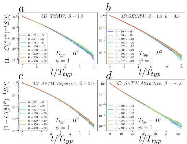
Figure 6. Asymptotic FPT distribution of non compact self-interacting random walks in confined domains for fresh initial conditions. Here S(t) is the survival probability of the random walker, whose scaling with geometrical parameters is deduced from (27). The collapse of numerical simulations after rescaling for different values of the geometrical parameters captures the dependence of the FPT distribution on r, R . Simulations are performed in 3d boxes of size R with reflecting boundary conditions and the constant C is measured numerically. a. 3d TSAW with \beta = 1.0 . b. 3d SESRW with \beta = 1.0 and k = 0.5 . 3d SATW repulsive with \beta = 3.0 (c) and with \beta = -1.0 (d).
