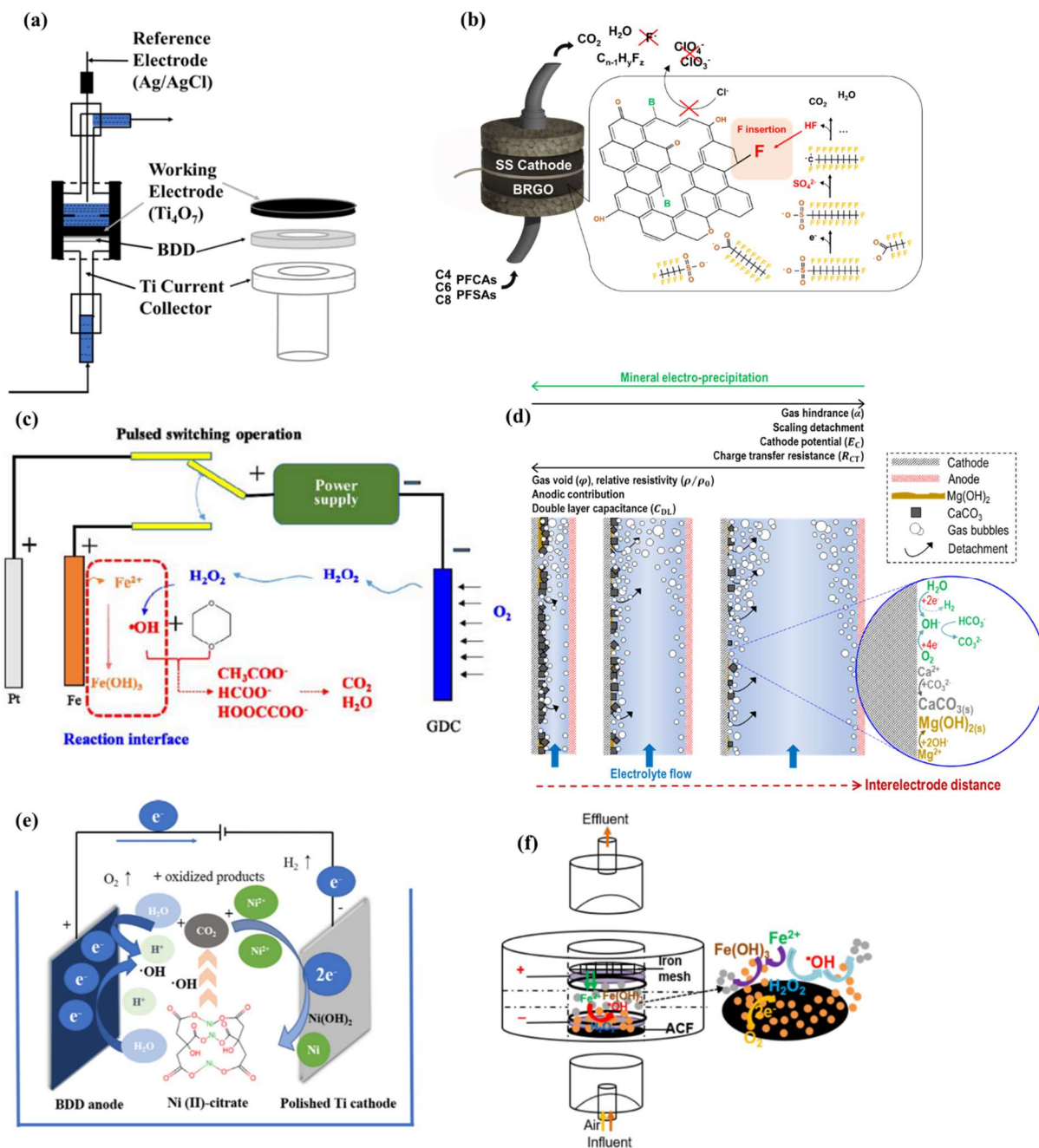
Fig. 1. Hybrid reactor setup implementing electro-separation/electro-conversion combinations in simultaneous operation: (a) electrofiltration/electrooxidation in flow-through parallel-plate system (Reproduced with permission from [10]. Copyright 2020, American Chemical Society), (b) electrosorption/electrooxidation in flow-through parallel-plate system (Reproduced with permission from [11]. Copyright 2022, Elsevier), (c) electrocoagulation/electro-Fenton in stirred tank reactor with electrodes in parallel (Adapted with permission from [13]. Copyright 2021, IWA Publishing), (d) electroprecipitation/electrooxidation in flow-by parallel-plate system (Adapted with permission from [23]. Copyright 2022, Elsevier), (e) electrodeposition/electrooxidation in stirred tank reactor with electrodes in parallel (Reproduced with permission from [24]. Copyright 2022, Elsevier), (f) Electrosorption/electrocoagulation/electro-Fenton in flow-through parallel-plate system (Reproduced with permission from [25]. Copyright 2021, Elsevier).
