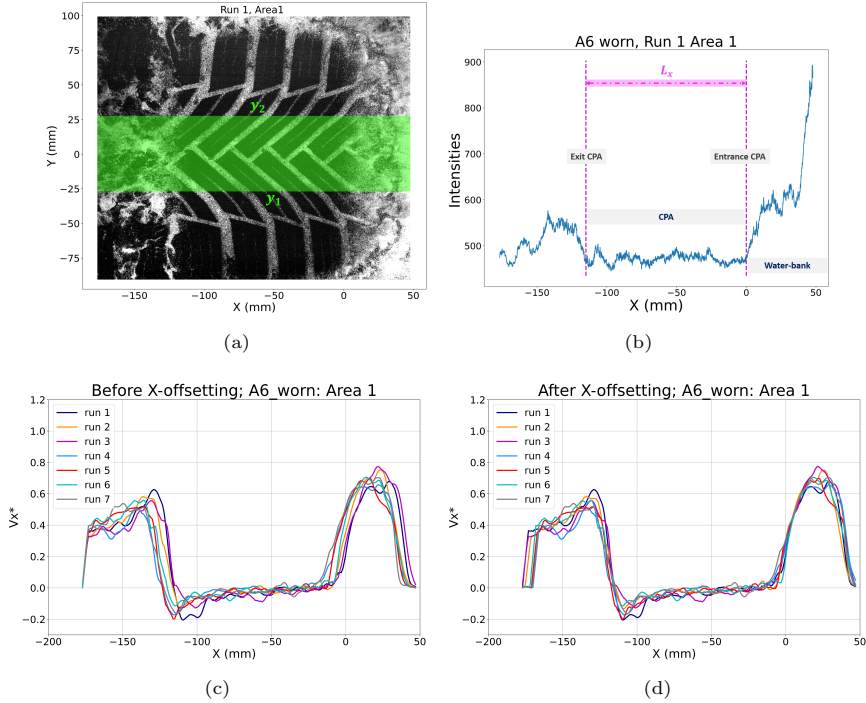
Fig. 5: Area 1 highlighted in green on raw image of the A6 at V_0=11.11m.s^{-1} and H_w = 1.5mm (a), image intensities space averaged along Y-axis in Area 1 (b) and V_{x^*} space averaged along Y-axis in Area 1 before (c) and after (d) X-offsetting
