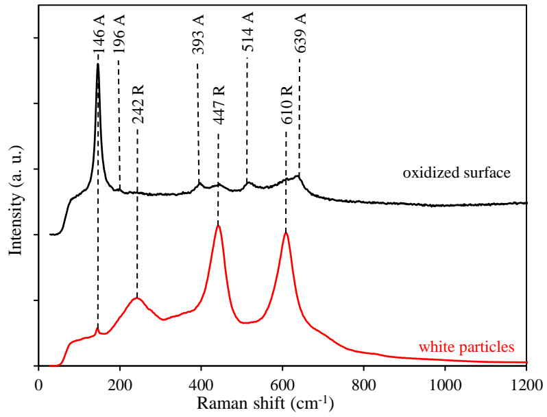
Figure B. Raman analysis of the laser-treated surface before US cleaning.
