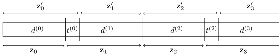
Figure 8: Decomposition of d in the case where the sequence (j_i) is (0, 1, 2, 3) .
