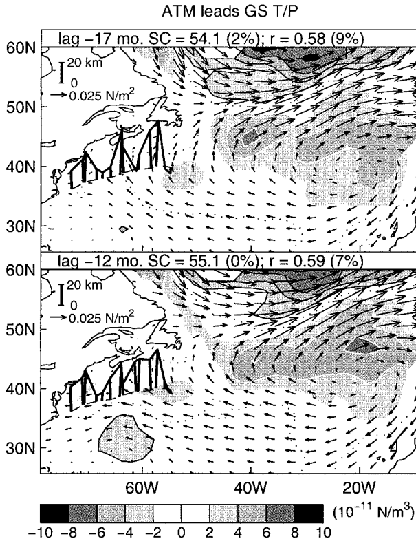
FIG. 8. First mode of the lagged MCA between T/P, wind stress, and wind stress curl at lag -17 and -12. Homogeneous maps are represented for the Gulf Stream path (see Fig. 7 for details) and heterogeneous ones for the atmosphere. The time series are normalized so that the maps indicate typical amplitudes. The correlation coefficient r and square covariance SC are given with estimated significance level. Positive (negative) contours are in black (white) and dots indicate zero.
