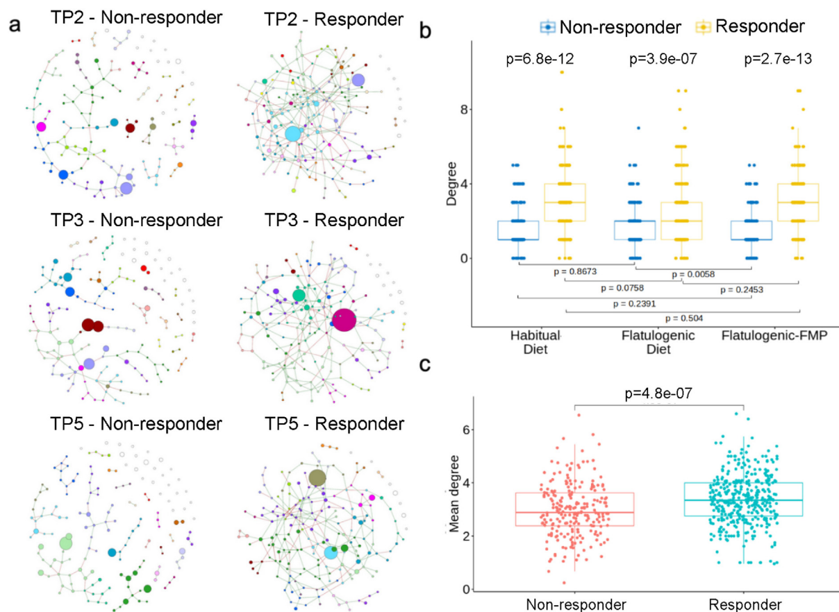
Fig. 6. Microbiome network analysis of responders ( n = 28 ) and non-responders ( n = 11 ) to the FMP. a) Network representation for responder and non-responder groups at three time points. A higher resolution of the labeled networks is available in Supplementary Fig. S8. b) Distribution of degrees (connections) between responders and non-responders over the three time points. c) Mean degrees obtained from randomization of an equal number of samples from each group to avoid bias that could be introduced by a different number of samples in each group and therefore a different number of processed mOTUs.
