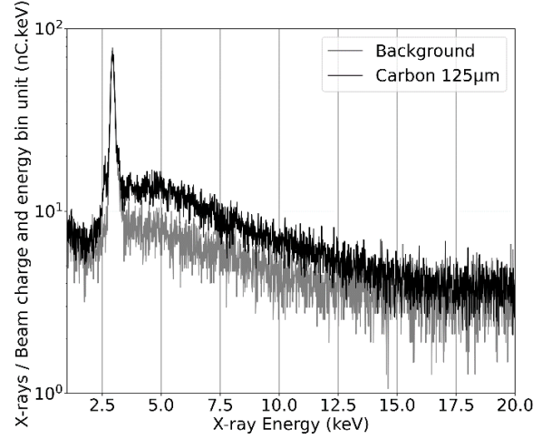
Figure 3. X-rays spectra from background and carbon with 39 MeV proton beam.
