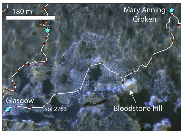
Figure 19. Detailed view of the traverse from the Glasgow drill hole to the Mary Anning drill hole. Background: HiRISE image ESP_060840_1750. The white line is the rover traverse path and the brown circles are stops along the traverse. The blue stars are drill locations. The text “sol 2783” marks where the mosaic in Figure 17 was obtained.
