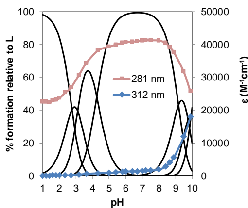
Fig. 3 Species distribution curves of compound H_3L_2 with molar extinction coefficients at the maximum absorption wavelengths ( C_L = 5.3 \times 10^{-5} M).
