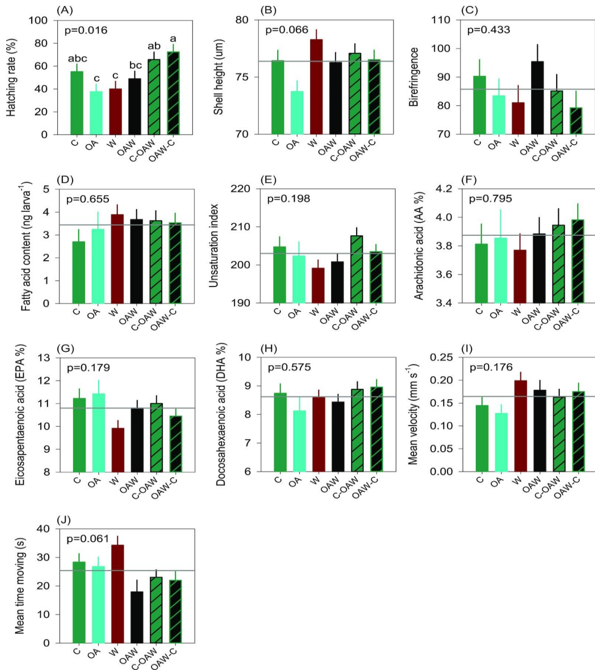
868 Figure 7. Hatching rate, shell height, birefringence (greyscale score), total fatty acid content and 869 essential fatty acid concentration (A-H), as well as velocity and motility (I, J). Data are least square 870 means \pm SE among tanks (n=3 or 6). Effects and p -values are shown when significant otherwise the 871 mean is shown by the grey line when non significant (NS). Abbreviations: C – control (21°C, ambient 872 pH), OA – ocean acidification (21°C, -0.33 pH unit), W – warming (24°C, ambient pH), OAW – ocean 873 acidification and warming (24°C, -0.33 pH unit).
