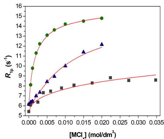
Figure 1. Relaxometric titrations (25 °C, 0.15 M NaCl) of the [Gd(CHXOCTAPA)] - complex with LaCl 3 (squares, C Lig = C Gd3+ =1.001 mM at pH=4.69), YbCl 3 (circles, C Lig = C Gd3+ =1.113 mM at pH=4.79) and ZnCl 2 (triangles, C Lig = C Gd3+ =1.001 mM at pH=4.81). All solutions were buffered using 50 mM dimethylpiperazine, DMP. The solid lines show the fit of the data for stability constant determination.
