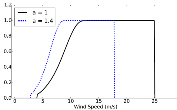
Figure A2. Power curve of a Vestas-90-2MW Turbine with normalized power.
