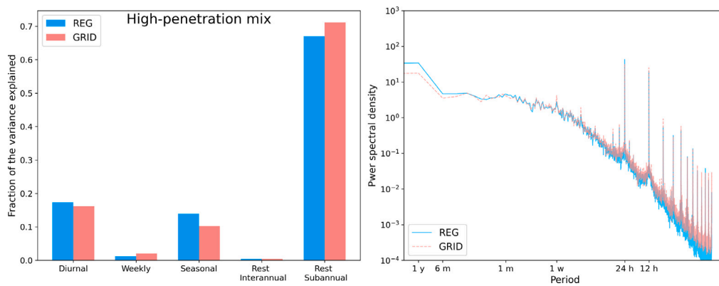
Fig. 7. Representation of the variance distribution in frequencies. On the left, the fraction of the variance of the high-penetration scenario explained by the daily, seasonal and weekly cycles and for all other frequencies for REG (blue) and GRID (red). On the right, the Welch estimate of the power spectral density for REG (blue) and GRID (red).
