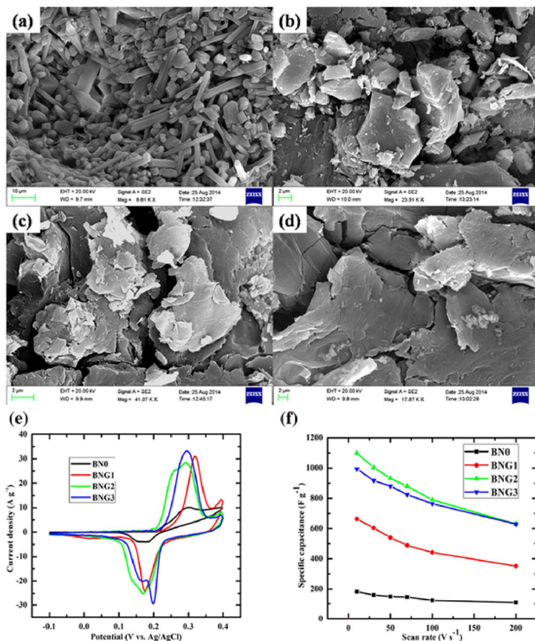
Fig. 16. FE-SEM images of (a) BNO, (b) BNG1, (c) BNG2, and (d) BNG3; (e) CV plots at 10 mV s -1 scan rate, and (f) variation of the specific capacitance with scan rate. Reprinted with permission of Saha et al.
