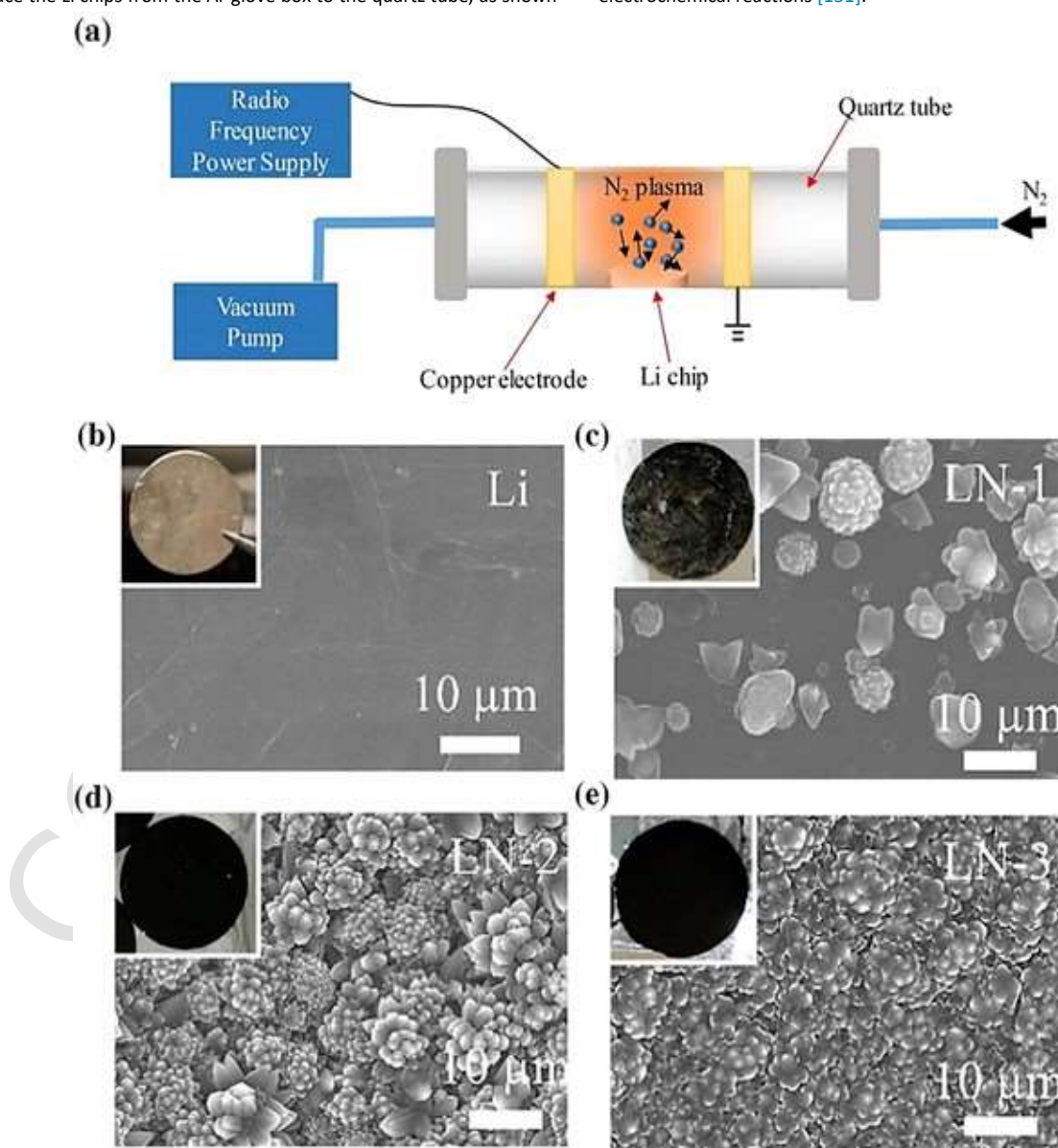
Fig. 13. (a) Experimental setup for the synthesis of \text{Li}_3\text{N} film electrode and SEM micrographs with the corresponding photos (in inset) of \text{Li}_3\text{N} films at varying times of \text{N}_2 plasma exposure. (b) Bare \text{Li} , (c) 1-min, (d) 2-min, and (e) 3-min plasma activation processing. Reprinted with permission of Chen et al.
