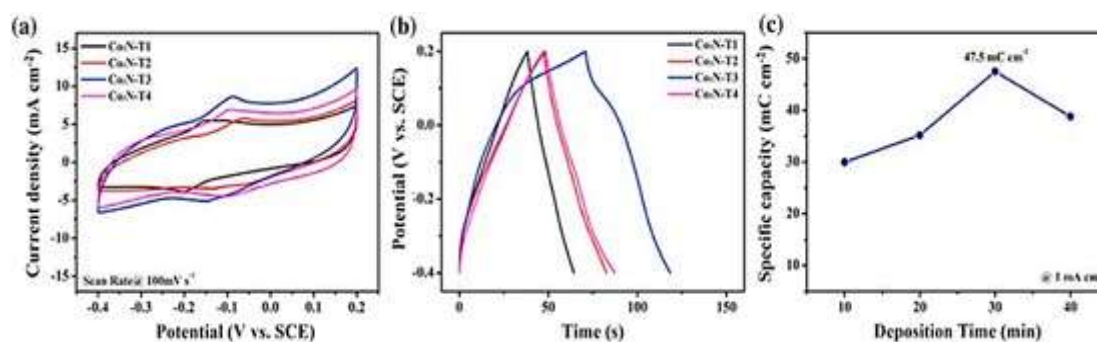
Fig. 9. Electrochemical properties of T1-T4 CoN thin film electrodes: (a) CV curves at 100 mV s -1 scan rate, (b) GCD curves, and (c) comparison of the specific capacity at 1.0 mA cm -2 . Reprinted with permission of Zhang et al.
