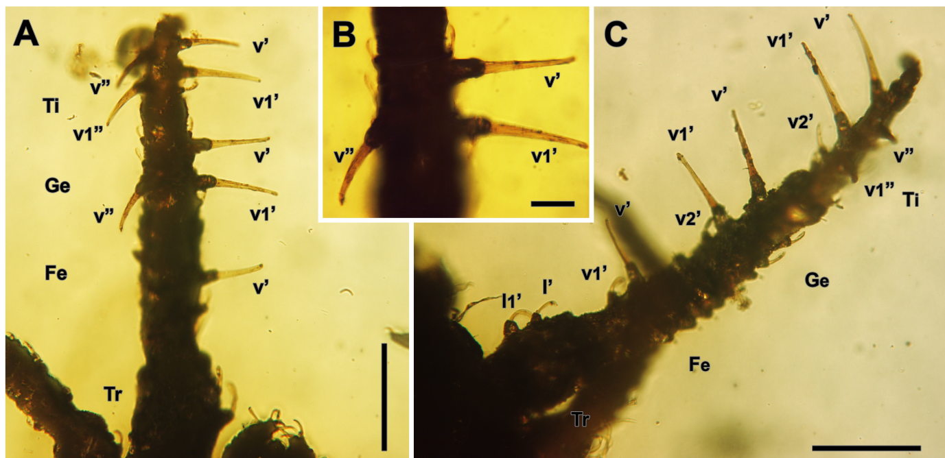
Figure 7 Caeculus fedrae sp. nov., Par2, A right leg I, ventral view; B same, detail of the spines of the ( v ) series of the genu; C right leg I, ventral view. Scale bars A, 200 \mu m; B, 50 \mu m; C, 200 \mu m.
