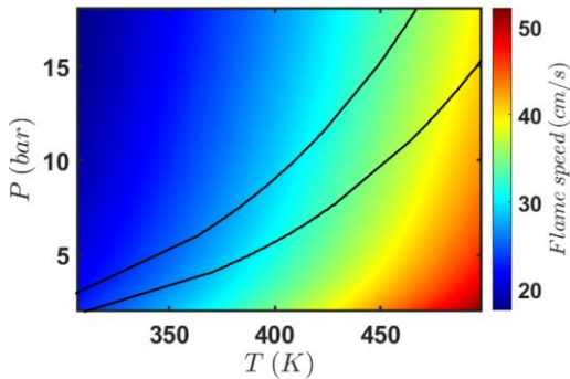
Fig. 4: S_u = f(P, T) correlation map at \varphi = 2.5
