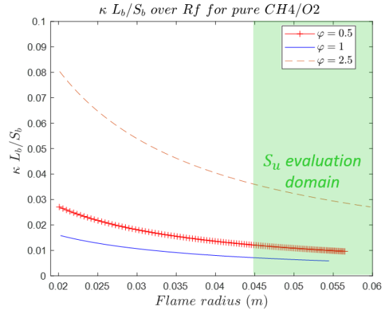
Fig. 1: \kappa L_b/S_b ratio over flame radius R_f for 2 different equivalence ratios ( \text{CH}_4/\text{O}_2 mixture)
