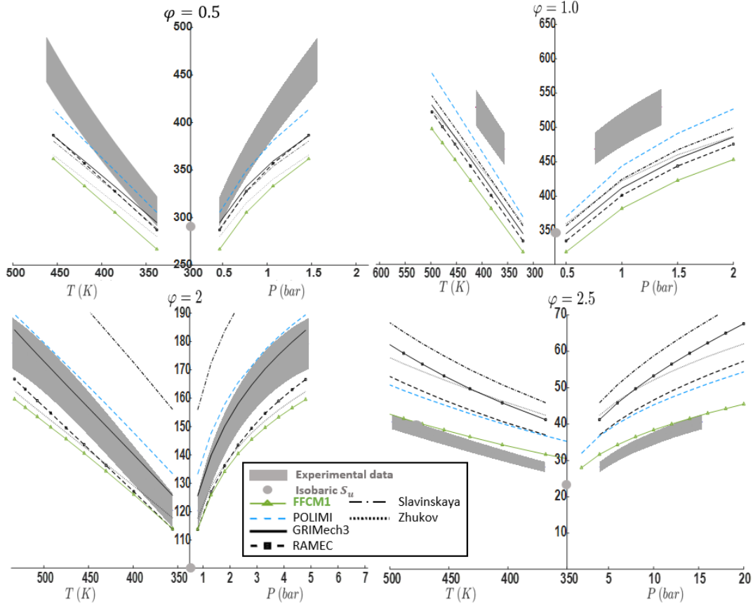
Fig. 2: Flame speed S_u [ \text{cm}\cdot\text{s}^{-1} ] for CH_4/O_2 mixtures at various equivalence ratios \varphi (thickened traces) as a function of T and P compared to several kinetic mechanisms (lines). Single symbols are for experimental isobaric flame speeds.
