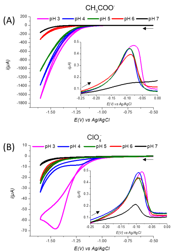
Fig. 2. Cyclic voltammograms recorded at 50 \text{ mV}\cdot\text{s}^{-1} at pH = 3, 4, 5, 6 and 7 in ammonium acetate (A) and \text{NaClO}_4 (B) Inset: enlargement of the copper stripping potential window.
