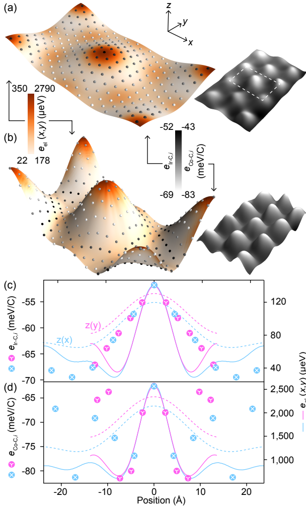
FIG. 2. (a,b) Spatial distribution of the elastic ( e_{el} evaluated on a square grid with 0.2 \text{ \AA} steps) and adhesion ( e_{Ir-C,i} , e_{Co-C,i} ) energy densities for graphene on Ir and Co/Ir, and corresponding STM topographs ( 9 \times 6.5 \text{ nm}^2 , one unit cell sketched with a dotted frame). The z scale is multiplied by 10. (c,d) Cross-sections, along x and y axes, of the membrane's height (dotted lines) and corresponding elastic (solid lines) and adhesion ('X' and 'Y' symbols) energies, for graphene/Ir (c) and graphene/Co/Ir (d).
