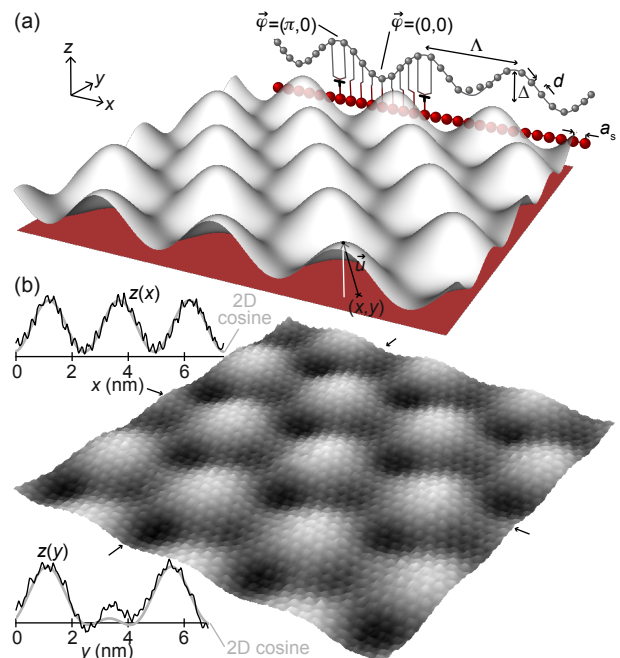
FIG. 1. (a) Points on the membrane are displaced from their position on a flat unrippled membrane by \vec{u}(x, y) . The cross-section (top-right) shows the moiré pattern's undulation (period \Lambda , amplitude \Delta ) and the atomic lattices (interatomic distances d and a_s in the membrane and substrate, respectively). The 2D phase \vec{\varphi} , i.e. the atomic stacking, varies from a valley to a hill. There, a substrate atom stands halfway between two membrane atoms ( \Upsilon symbols). (b) STM topograph ( 8 \times 8 \text{ nm}^2 ) of a graphene membrane onto Ir(111), and apparent height profiles extracted between the arrows fitted using a cosine function.
