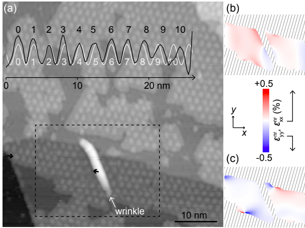
FIG. 3. (a) STM topograph of graphene/Ir intercalated with a Co submonolayer. A graphene wrinkle appears as a bright linear feature. Inset: apparent height profile between the two black arrows, compared to a sinusoid (the successive maxima are numbered). (b,c) Maps of the moiré lattice compression/expansion in the xy plane, roughly perpendicular (c) and parallel (d) to the wrinkle.
