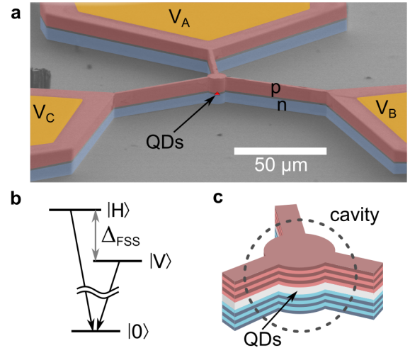
Figure 1. (a) SEM image of a 10 μm diameter micropillar cavity with QDs embedded at its center. Ridges connect the pillar to three electrical contacts defined via gold pads. The image has been artificially colored to evidence the different components of the structure (b) Schematic of the exciton energy levels. (c) Schematic zoom of the pillar structure highlighting the top and bottom cavity mirrors defining the cavity in the vertical direction. The QD layer is vertically centered in the cavity.
