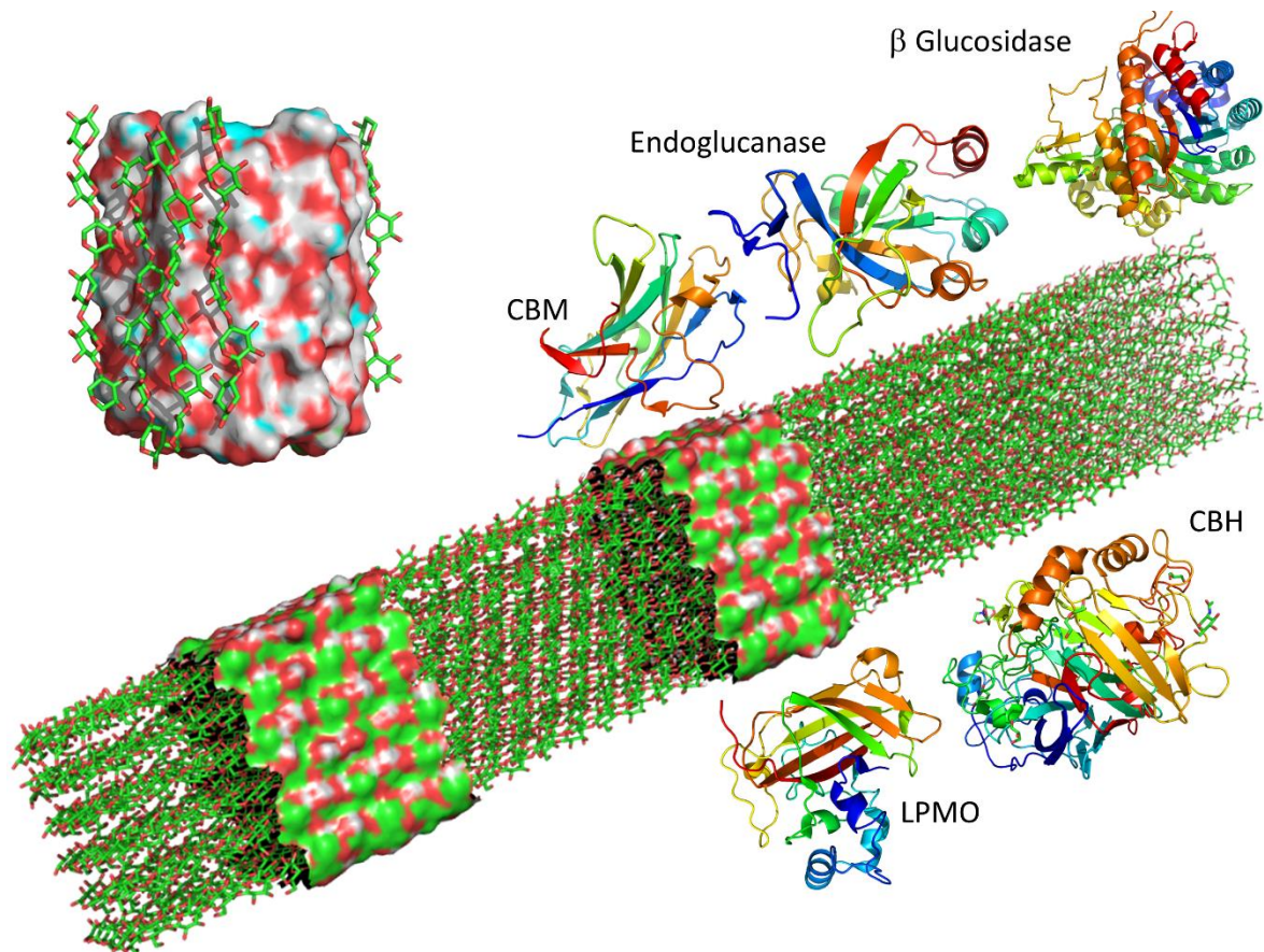
Figure 27. Interaction and deconstruction of cellulose. The middle portion of the figure shows an idealized construction of the parallel arrangement of 36 cellulose chains constructed for an MD simulation with full consideration of hydration. The water molecules are not displayed. Two sections of the microfibrils display the van der Waals surface to highlight the potential for interactions. The left-hand side panel displays the interactions between the cellulose microfibril and xylan (one of the constituents of the plant cell) resulting from a molecular modeling study. 305 The figure shows the three-dimensional structures of the representative cellulolytic enzymes degrading cellulose down into glucose: endoglucanase, cellobiohydrolase, and \beta -glucosidase. They follow the action of the carbohydrate-binding module and lytic polysaccharide monooxygenases (LPMOs), which significantly enhance cellulose breakdown. CBM, PDB: 4B96; endoglucanase, PDB: 5XBU;442 \beta -glucosidase PDB 3WH5;443 CBH, PDB: 505D;444LPMO, PDB: 6RW7445. Reproduced from ref 5. Copyright 2021 Elsevier
