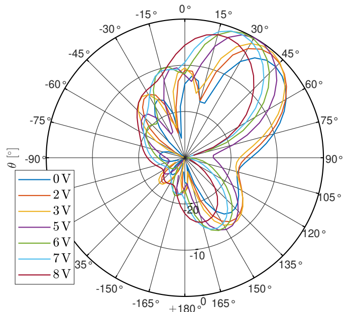
Fig. 5. Realized normalized gain at 7.75GHz in H-plane( \Phi = 90^\circ ) for different bias
