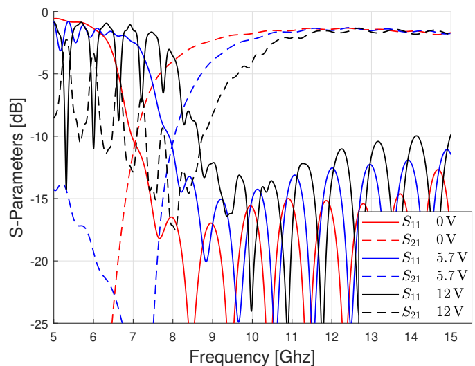
Fig. 2. Simulated S-Parameters for 3 different bias
