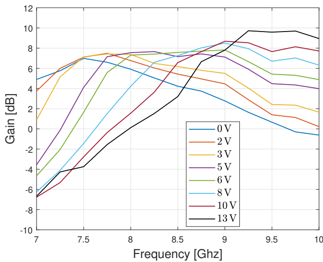
Fig. 10. Maximum measured gain for different configurations
