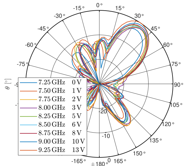
Fig. 11. Measured normalized gain for a fixed beam in H-plane ( \Phi = 90^\circ ) at 35^\circ \pm 2^\circ over frequency
