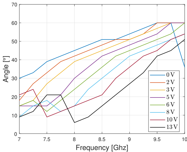
Fig. 9. Main beam angle for different configurations
