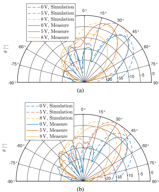
Fig. 7. Comparison between simulated and measured gain in H-plane for different bias: (a) both at 7.75 GHz and (b) simulated results are at 7.75 GHz and measured result are at 8 GHz taking into account the frequency shift
