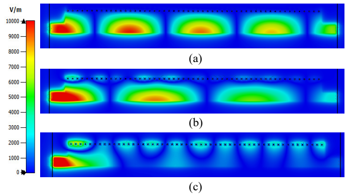
Fig. 1. Electric field distributions along the waveguide ( z = 0.25 mm) at 8GHz for three different voltages: (a) 0 V, (b) 4.7 V and (c) 12 V
