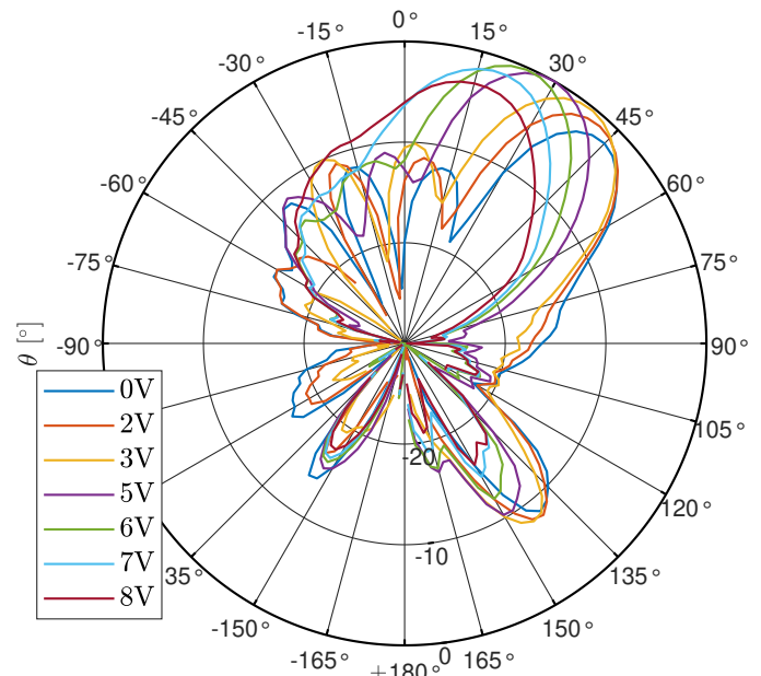
Fig. 8. Measured normalized gain at 8 GHz in H-plane ( \Phi = 90^\circ ) for different bias
