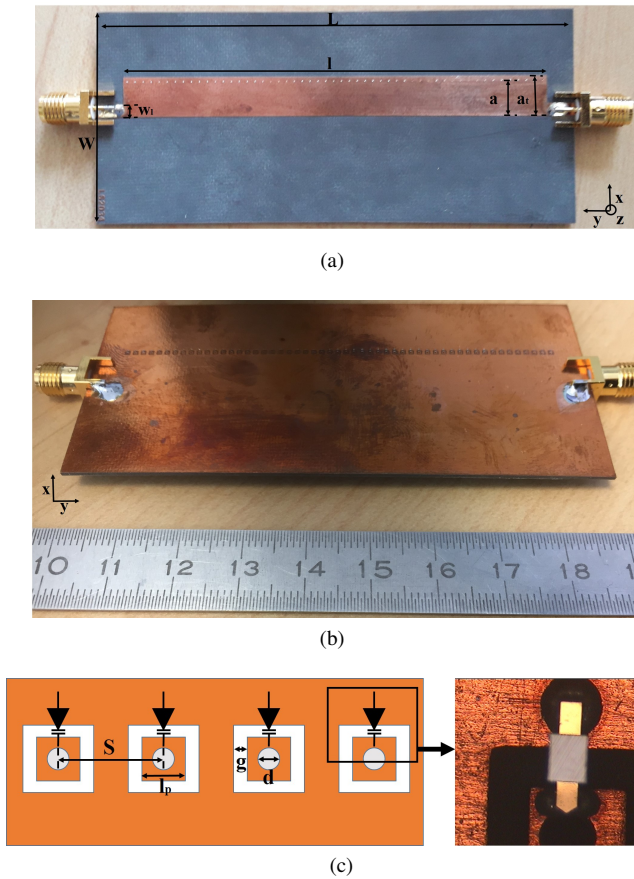
Fig. 3. Antenna prototype: (a) Top view, L = 89.5 mm, W = 40 mm, l = 79.5 mm, a = 7.25 mm, a_t = 8 mm, w_l = 2.4 mm, (b) bottom view and (c) Varactor placement, g = 0.2 mm, d = 0.3 mm, l_p = 0.6 mm, S = 1.5 mm
