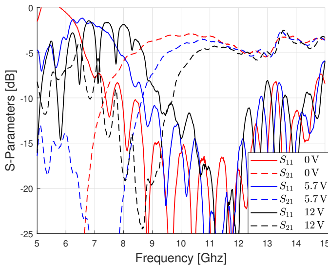
Fig. 6. Measured S-Parameters for 3 different bias
