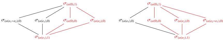
Figure 5. Comparison of \Sigma_{V^j, i'} in Lemma 5.1.6 when \tilde{w}_{i'}^* t_{-1} = \alpha .
