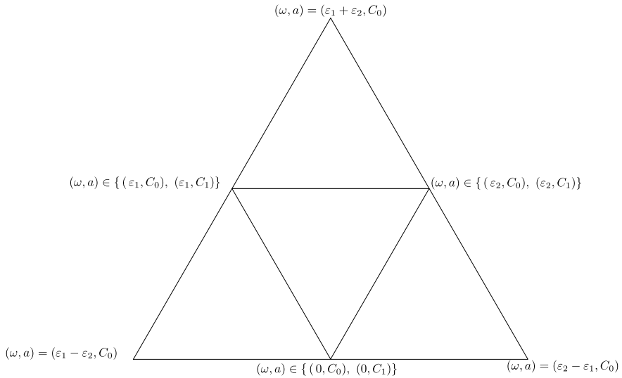
Figure 1. The set \Sigma_0 .
