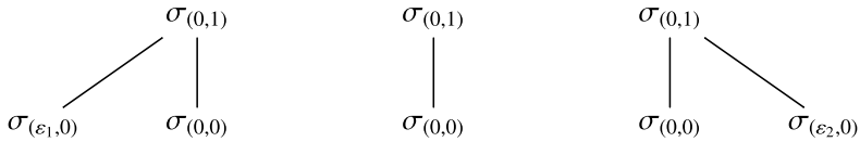
Figure 3. Comparison of \Sigma_{V^j, i'} in Lemma 5.1.4.
