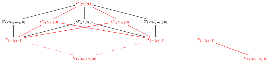
Figure 7. Comparison of \Sigma_{V^j, i'} in Lemma 5.1.7 when \tilde{w}_i^* t_{-1} = \gamma^+ .
