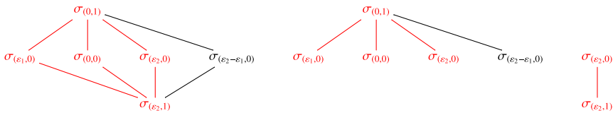
Figure 4. Comparison of \Sigma_{V, i'} and \Sigma_{V^j, i'} in Lemma 5.1.5 when \tilde{w}_{i'}^* t_{-1} = \text{id} .
