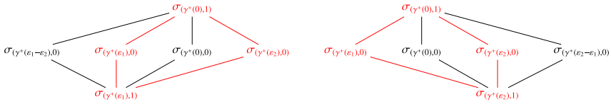
Figure 6. Comparison of \Sigma_{V^j, i'} in Lemma 5.1.6 when \tilde{w}_i^* t_{-1} = \gamma^+ .
