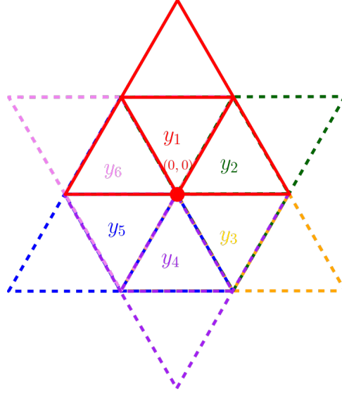
FIGURE 2. Case where W_{\text{obv}}(x^*) = \{(0,0)\} and \#S(x^*) = \#W . The set W_{\text{obv}}(x^*) is pictured by the red dot and the set S(x^*) by the 6 triangles. The simple walks only produce new specializations.
