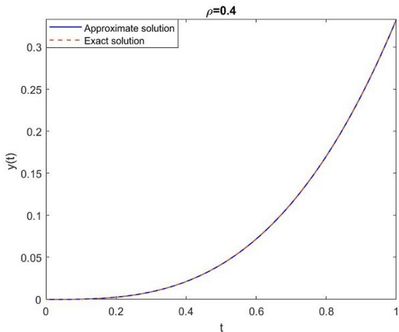
Figure 1. Numerical simulation for Cauchy problem for \rho = 0.4 .
