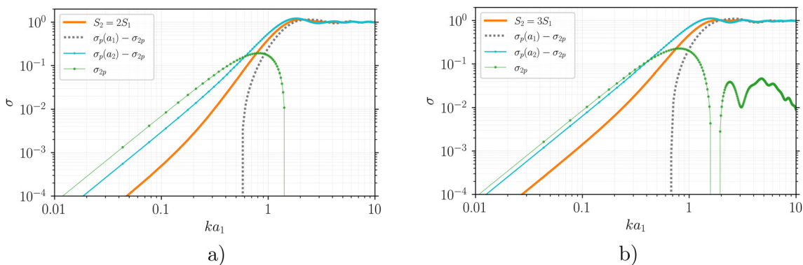
FIG. 11. (Color online) Dipole when one of the piston’s area is (a) twice that of the other, (b) triple that of the other.
