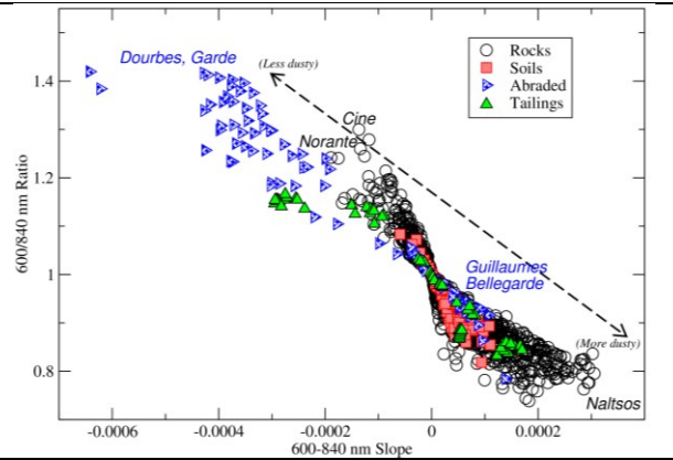
Fig. 6. Comparison of 600-840 nm slope and ratio with abraded targets and representative endmembers noted [cf. 8].
