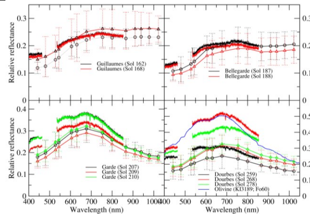
Fig. 3. SuperCam VIS spectra for abraded rock targets from the Cf-fr unit ( Guillaumes , Bellegarde ) and Séítah ( Garde , Dourbes ), and ZCAM spectra from the same regions (std. deviations shown). USGS lab olivine spectrum also shown.
