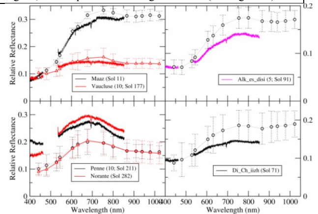
Fig. 4. SuperCam VIS spectra for representative rock targets (raster location # listed unless spectrum is raster average).
