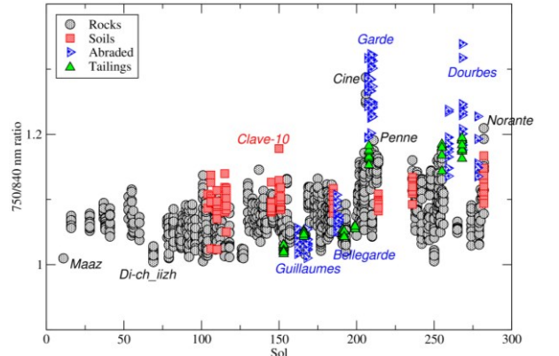
Fig. 2. 750/840 nm ratios (sensitive to ferrous minerals) from SuperCam VIS spectra for target classes shown in legend, with representative targets labeled (see Figs. 3-5).
