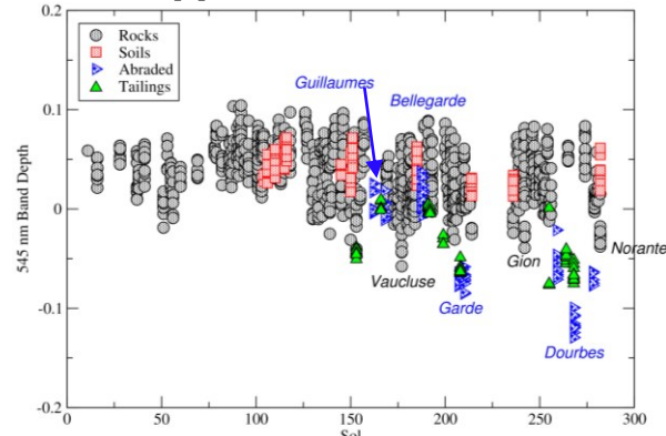
Fig. 1. 545 nm band depths (sensitive to crystalline Fe^{3+} ) from SuperCam VIS spectra for target classes shown in legend, with representative targets labeled (see Figs. 3-5).
