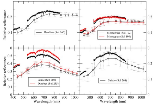
Fig. 5. Average SuperCam VIS spectra for abrasion and coring tailings from the Cf-fr unit ( Roublion , Montdenier , Montagnac ) and Séítah ( Garde , Dourbes , Salette ), and ZCAM spectra from the same regions (std. deviations shown).
