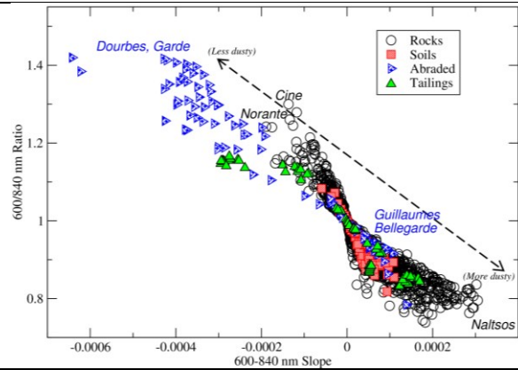
Fig. 6. Comparison of 600-840 nm slope and ratio with abraded targets and representative endmembers noted [cf. 8].
