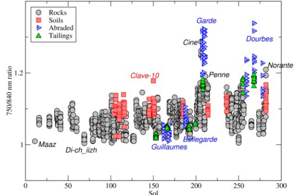
Fig. 2. 750/840 nm ratios (sensitive to ferrous minerals) from SuperCam VIS spectra for target classes shown in legend, with representative targets labeled (see Figs. 3-5).
