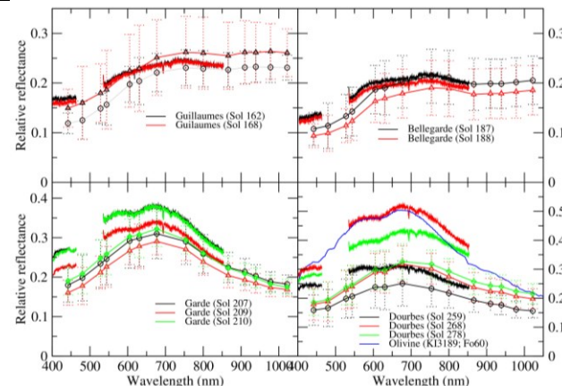
Fig. 3. SuperCam VIS spectra for abraded rock targets from the Cf-fr unit ( Guillaumes, Bellegarde ) and Séítah ( Garde, Dourbes ), and ZCAM spectra from the same regions (std. deviations shown). USGS lab olivine spectrum also shown.
