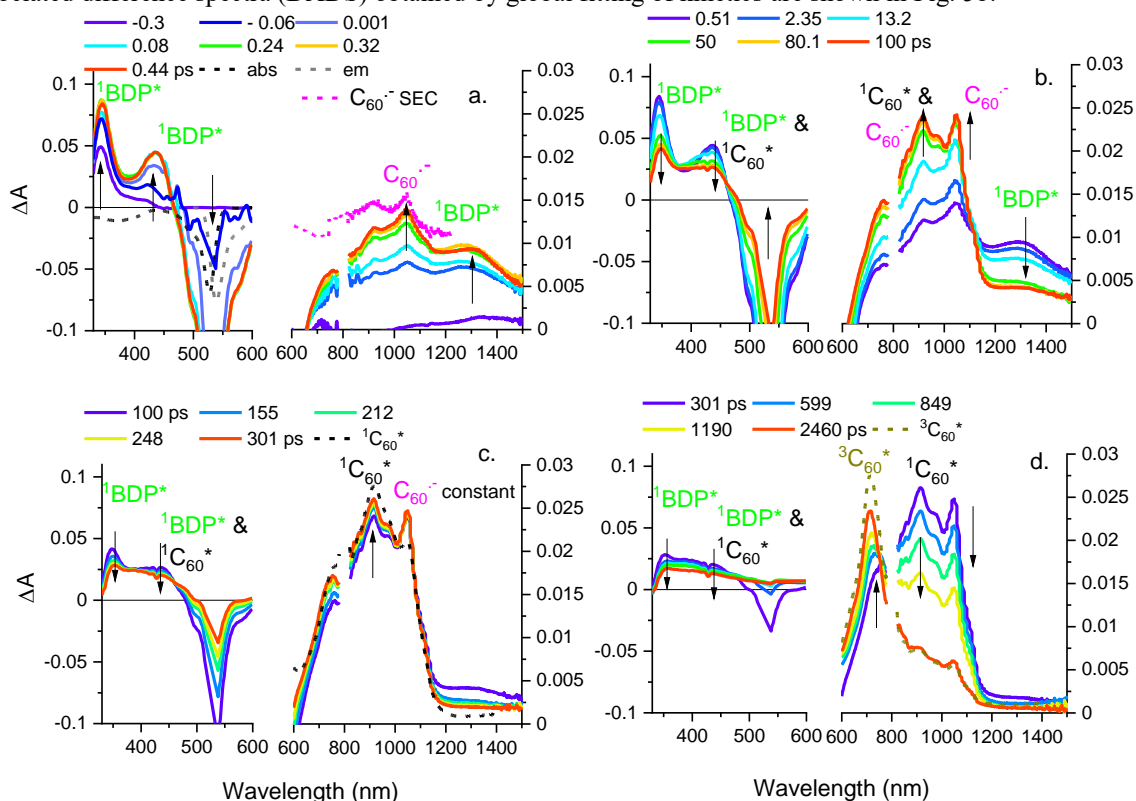
Fig. 4. Femtosecond transient absorption spectra of BDP- C_{60} at specified delay times: a. -0.3 to 0.44 ps; b. 0.51 to 100 ps; c. 100 to 301 ps and d. 301 to 2460 ps in deaerated benzonitrile. \lambda_{exc} = 525 nm. The grey and black curves in panel (a) represent the respective steady-state absorption (abs) and emission (em) spectra of pristine BDP.
