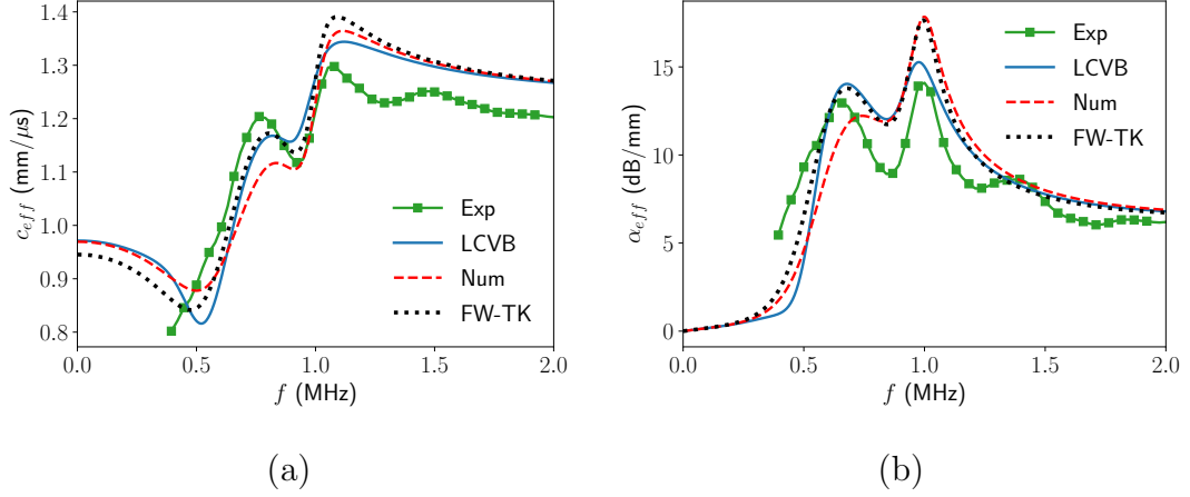
Figure 3: Concentration c = 6.4\% of tungsten carbide spheres in an epoxy matrix. (a) Phase velocity and (b) attenuation of the quasi-transverse coherent wave. Green line with squares: experiment, from Ref. [38], black dotted line: from Eq.(36) of Refs. [30, 29], blue solid line: from Eqs. (60), red dashed line: from Eq. (59)
