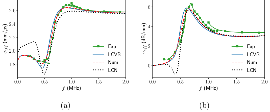
Figure 2: Concentration c = 5\% of tungsten carbide spheres in an epoxy matrix. (a) Phase velocity and (b) attenuation of the quasi-longitudinal coherent wave. Green line with squares: experiment from Ref. [55], black dotted line: from Eq.(36) of Ref. [31], blue solid line: from Eq. (57), dashed red line: from Eq. (56).
