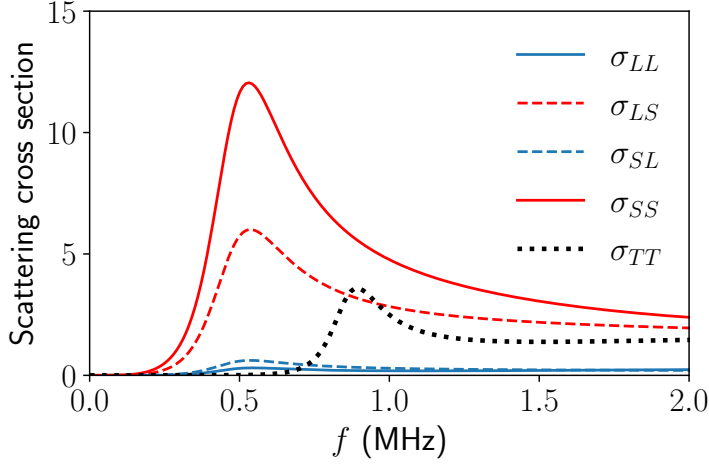
Figure 1: Tungsten carbide sphere in an epoxy resin : scattering cross sections \sigma_{IM} for an incident wave of type I and a scattered wave of type M .
