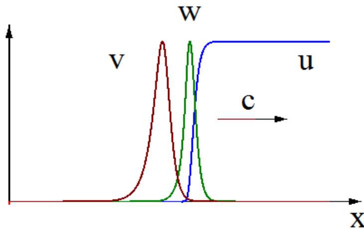
Figure 1. A snapshot of numerical solution of system (11)–(13). Infection spreads as a reaction-diffusion wave with a speed c , U(x, t) = u(x - ct) , I(x, t) = w(x - ct) , V(x, t) = v(x - ct) . Note that u_f = 0 here.
