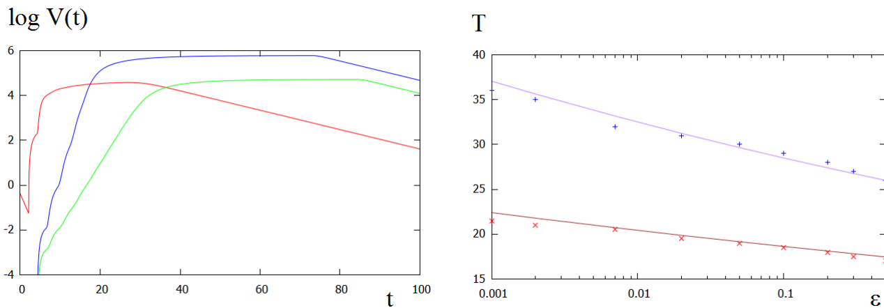
Figure 5. Left: V_1(t) (red) and V_2(t) (green) in the logarithmic scale for b_2 = 8 \times 10^4 ; V_2(t) (blue) for b_2 = 8 \times 10^5 . Right: transition time T as a function of mutation rate \epsilon for b_2 = 8 \times 10^4 (upper curve, crosses) and b_2 = 8 \times 10^5 (lower curve, crosses). Smooth lines represent analytical approximation with the functions p/\epsilon^q , p = 25, q = 0.057 (upper curve), p = 17, q = 0.04 (lower curve). The values of parameters: a_1 = 0.01, a_2 = 0.1, b_1 = 8 \times 10^4; D_1 = D_2 = 10^{-3}, \beta_1 = \beta_2 = 0.1, \sigma_1 = \sigma_2 = 1, \tau = 2, u_0 = 1, i_{10} = i_{20} = 0, v_{1,0} = 4.5, v_{2,0} = 0, x_0 = 0.1 .
