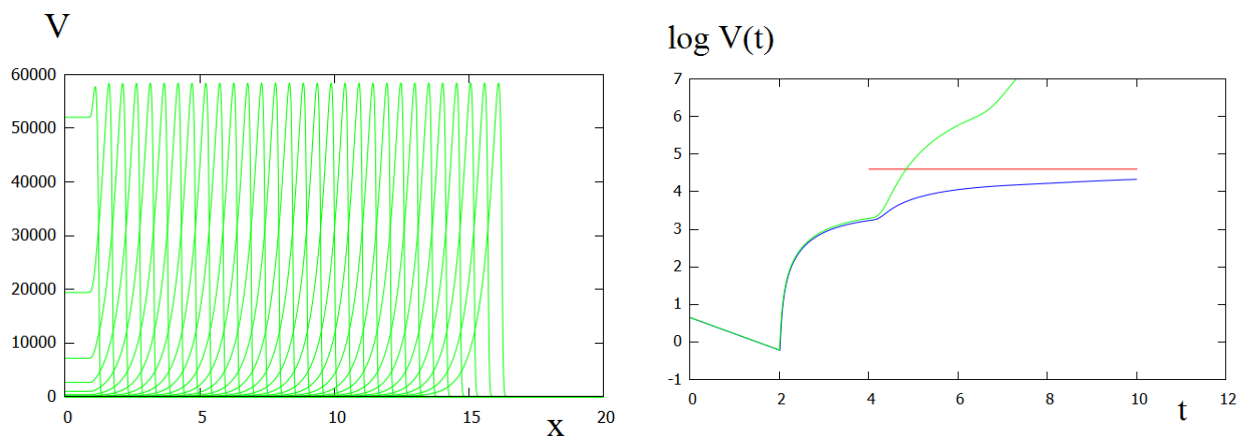
Figure 3. Left: virus distribution in consecutive moments of time (every 1 h). Right: total viral load W(t) = \int_0^L V(x,t)dx (in the logarithmic scale) found as solution of system (64), (65) (green), of system (11)–(13) (blue) and by the formula in Theorem 1 (red). The values of parameters: a = 0.01, b = 8 \times 10^4, D = 10^{-3}, \beta = 0.1, \sigma = 1, \tau = 2 .
