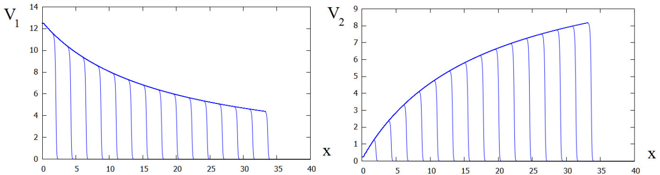
Figure 2. Numerical simulations of system (29)–(33) in the case where a_1 = a_2, b_1 = b_2 . Both virus spread in the form of waves, but the concentration of the first virus slowly decreases while of the second virus increases. The values of parameters: a_1 = 0.01, a_2 = 0.01, b_1 = b_2 = 80,000; D_1 = D_2 = 10^{-3}, \beta_1 = \beta_2 = 0.1, \sigma_1 = \sigma_2 = 1, \tau = 2, u_0 = 1, i_{10} = i_{20} = 0, v_{1,0} = 4.5, v_{2,0} = 0, x_0 = 0.1 .
