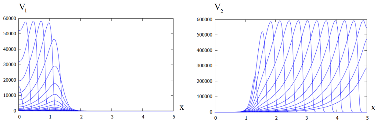
Figure 4. Distributions of V_1(x,t) (left) and V_2(x,t) (right) in numerical simulations of system (29)–(33). In the beginning of simulations, there is only the first virus variant. After some time, the second variant completely eliminate the first one. The values of parameters: a_1 = 0.01, a_2 = 0.1, b_1 = b_2 = 8 \times 10^4, D_1 = D_2 = 10^{-3}, \beta_1 = \beta_2 = 0.1, \sigma_1 = \sigma_2 = 1, \tau = 2, u_0 = 1, i_{10} = i_{20} = 0, v_{1,0} = 4.5, v_{2,0} = 0, x_0 = 0.1 .
