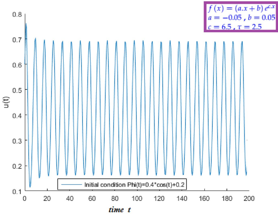
Fig. 4 Oscillations in time for f(u) = (-0.05.u + 0.05)e^{6.5.u}
