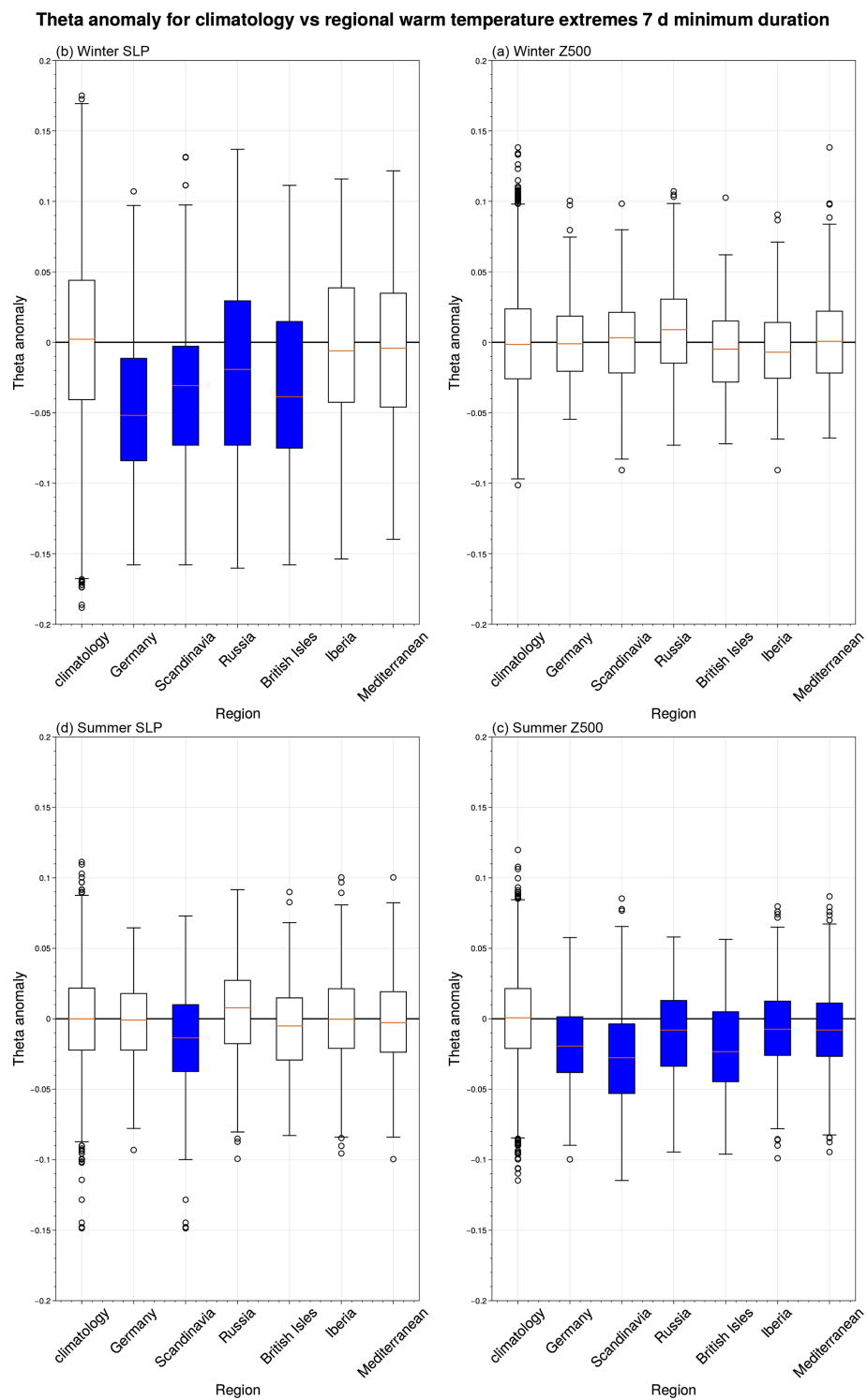
Figure A2. \theta ( \text{d}^{-1} ) anomaly box plots as in Fig. 3 but for a heatwave or warm spell of at least 7 d in duration.
