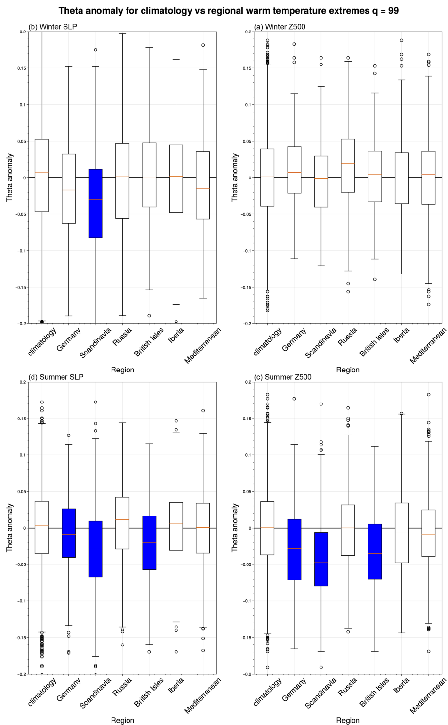
Figure A9. \theta ( \text{d}^{-1} ) anomaly box plots as in Fig. 3 but using the 99th percentile of the distribution of negative-log distances to define analogues.
