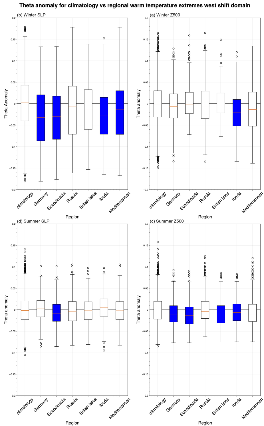
Figure A5. \theta ( \text{d}^{-1} ) anomaly box plots as in Fig. 3 but with a westward-shifted domain covering -50 – 35^\circ E.
