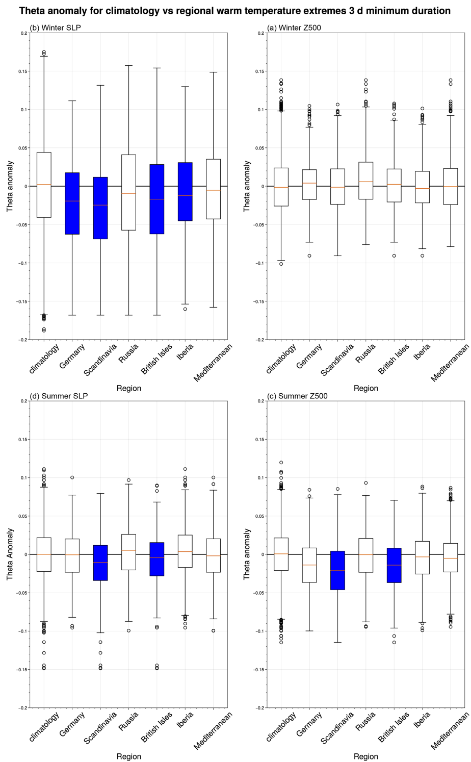
Figure A1. \theta ( \text{d}^{-1} ) anomaly box plots as in Fig. 3 but for a heatwave or warm spell of at least 3 d in duration.
