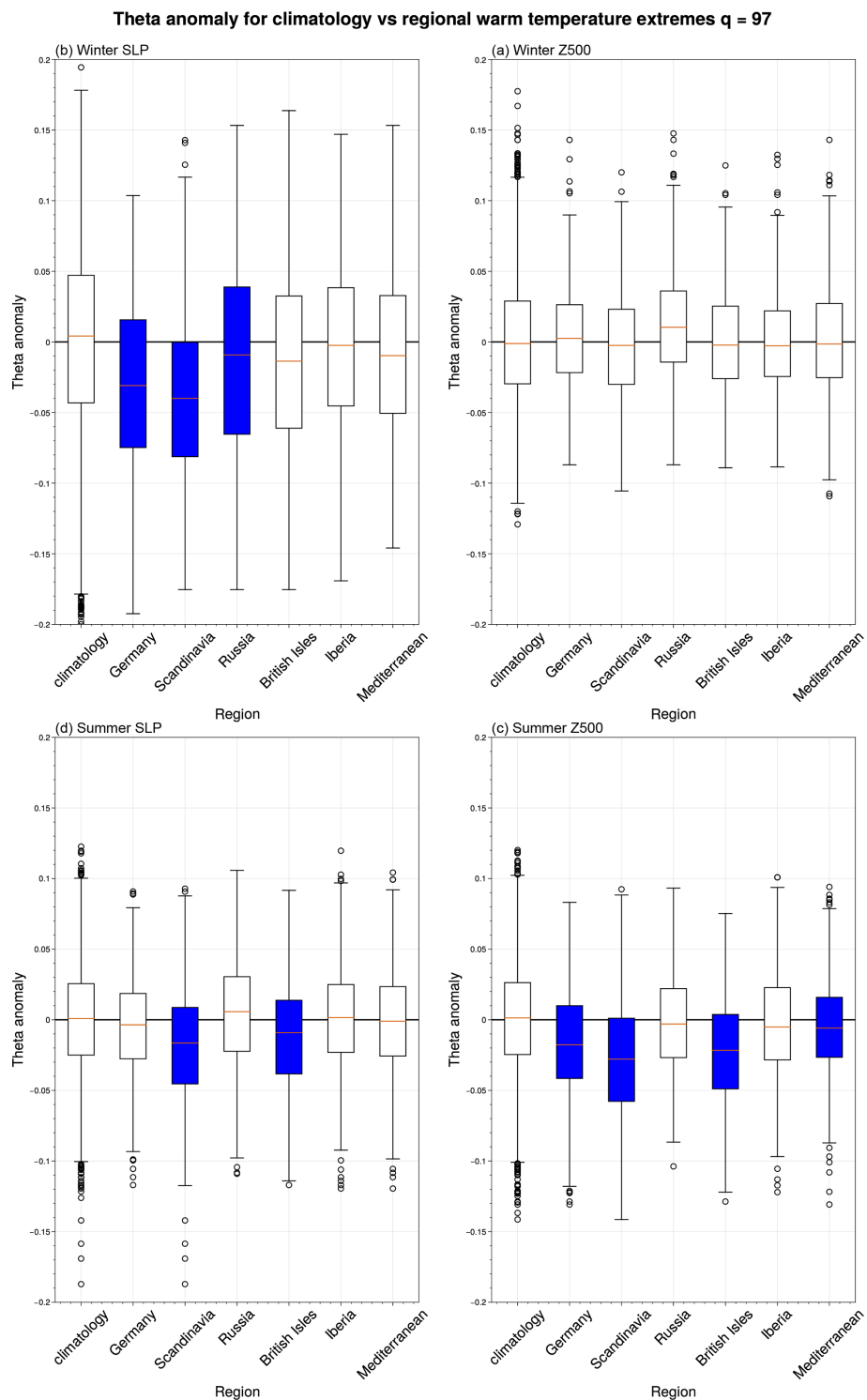
Figure A8. \theta ( \text{d}^{-1} ) anomaly box plots as in Fig. 3 but using the 97th percentile of the distribution of negative-log distances to define analogues.
