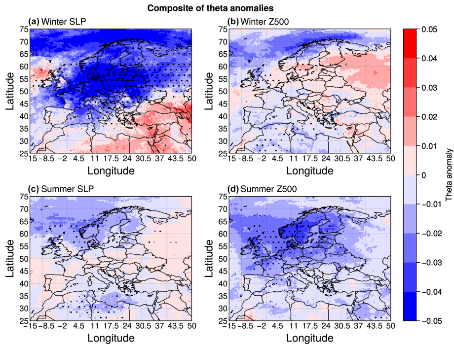
Figure 2. \theta ( \text{d}^{-1} ) anomalies for all warm-spell or heatwave days for each grid box during winter (a, b) and summer (c, d), where \theta has been calculated using SLP fields in (a) and (c) and Z500 fields in (b) and (d). Statistical significance is assessed as described in Sect. 2 and shown with stippling.
