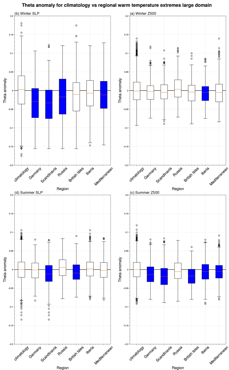
Figure A7. \theta ( \text{d}^{-1} ) anomaly box plots as in Fig. 3 but with a larger domain covering -20 – 55^\circ E.
