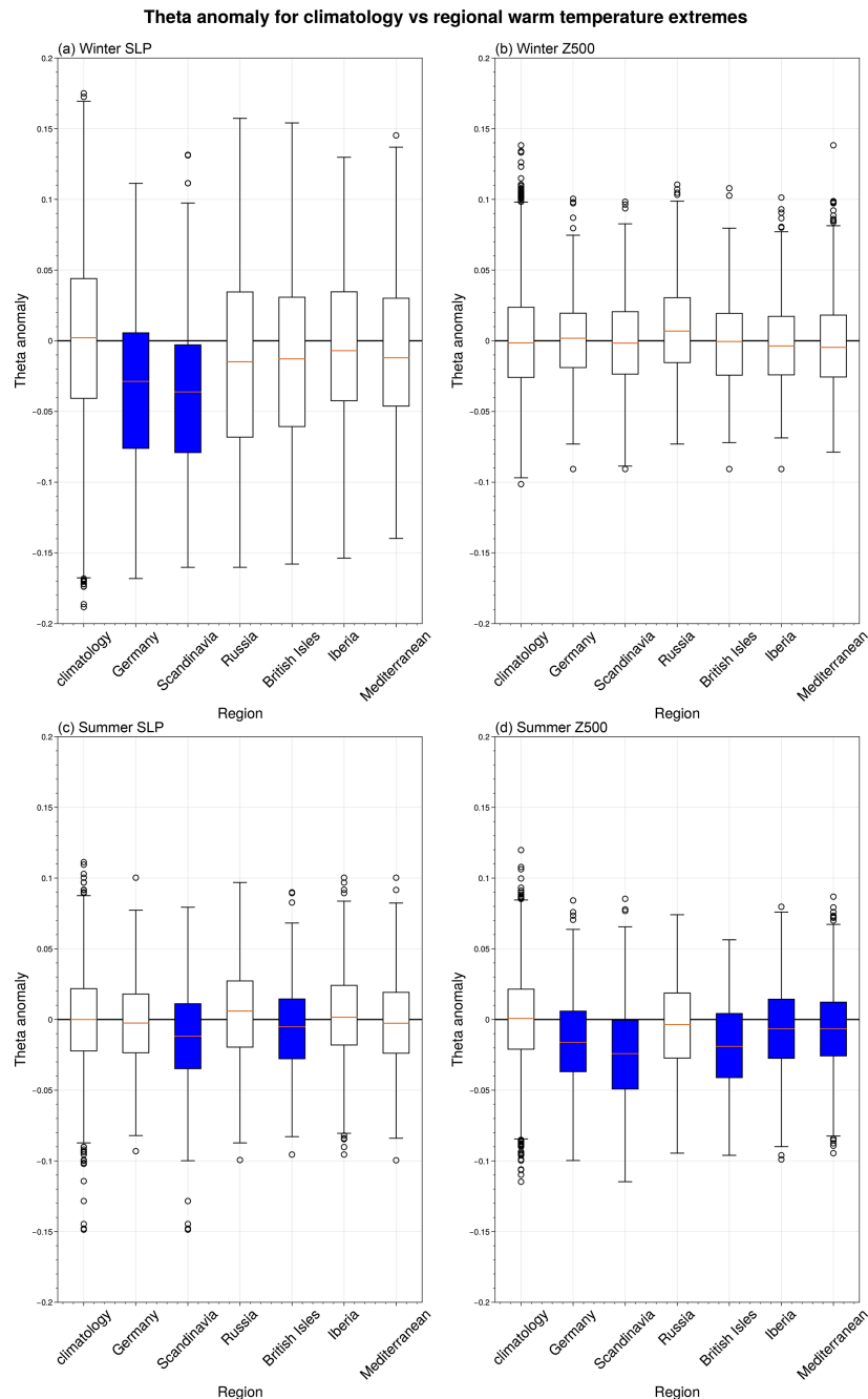
Figure 3. Box plots of \theta ( \text{d}^{-1} ) anomalies for all heatwave (c, d) or warm-spell (a, b) days in the considered regions at both the surface level (a, c) and the mid-level (b, d). Blue boxes indicate statistical significance, assessed as described in Sect. 2.
