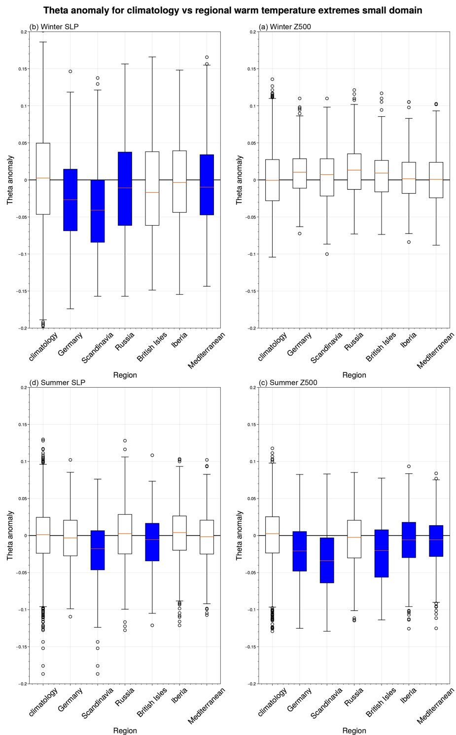
Figure A6. \theta ( \text{d}^{-1} ) anomaly box plots as in Fig. 3 but with a smaller domain covering -10 – 45^\circ E.
