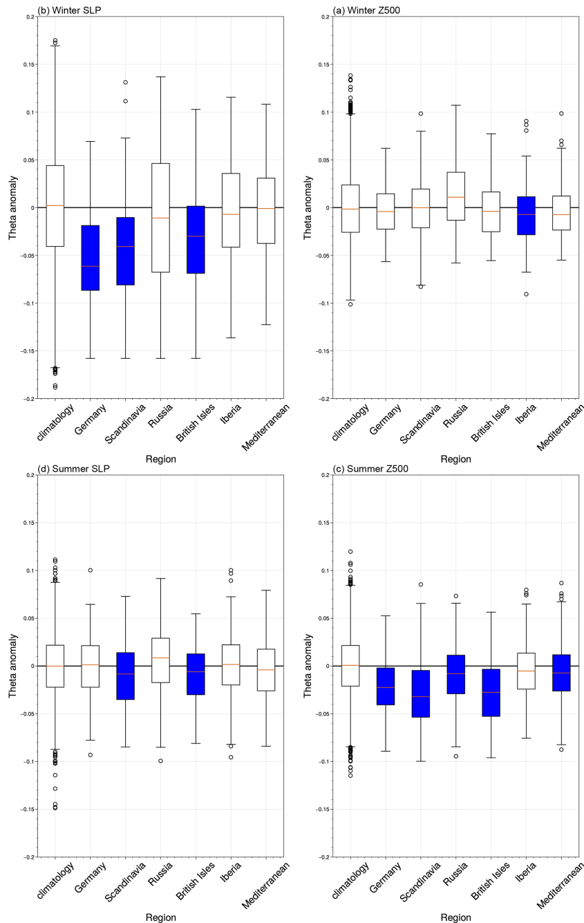
Figure A3. \theta ( \text{d}^{-1} ) anomaly box plots as in Fig. 3 but for warm-temperature extremes defined using temperatures above the local 95th percentile.
