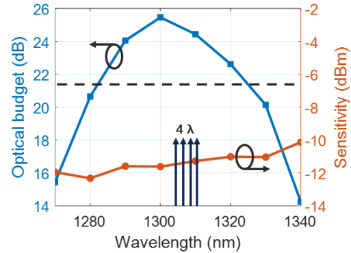
Fig. 3: Optical budget (blue square curve) and sensitivity at FEC threshold (red circle curve) of the Rx versus the wavelength of Ch 2.
