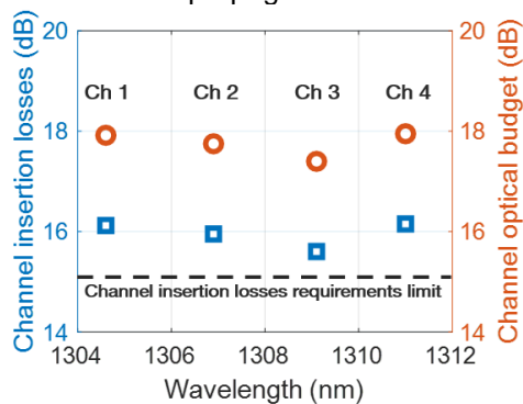
Fig. 6: Channel insertion losses (blue squares) and channel optical budgets (red circle) for the four channels in BtB.
