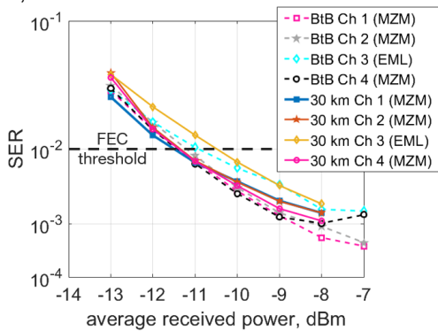
Fig. 5: SER versus average received optical power measured on point E in BtB (dash curve) and after 30 km of SSMF (full curve) for Ch 1, Ch 2 and Ch 4 (MZM) and Ch 3 (EML).
