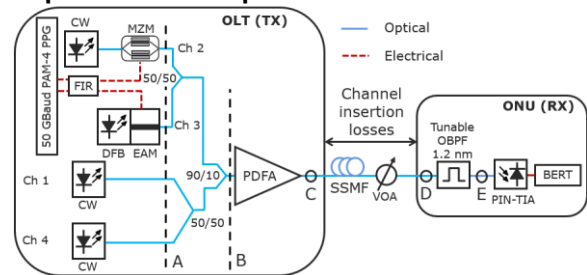
Fig. 1: Experimental setup.
