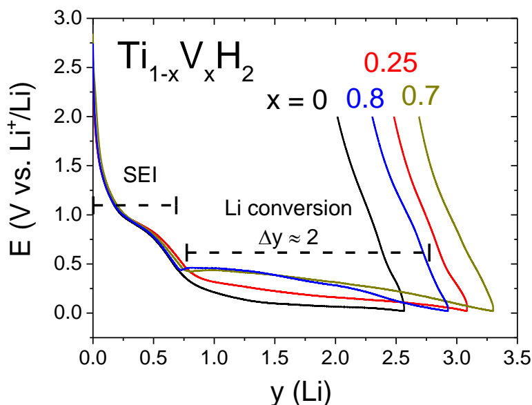
Figure 3 : Potential profiles of selected dihydrides \text{Ti}_{1-x}\text{V}_x\text{H}_2 during the first galvanostatic cycle in Li-ion half-cell.
