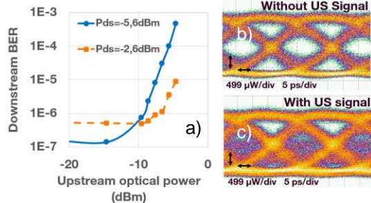
Fig. 5: BER measured on the DS for different US power injected in the SOA a), eye diagram without (b)) and with (c)) US signal in the SOA.
