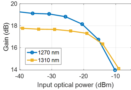
Fig. 2: Gain versus SOA input power at 280 mA and 20°C. After amplification, the DS signal crosses another CWDM filter (CWDM2) and reaches a variable optical attenuator (VOA1). The direct detection is realized by a photodiode (PD) PIN-TIA with 42 GHz 3 dB electro-optical bandwidth (EO-BW). The electrical signal is sent to the error detector (ED1) for bit error rate (BER) measurement. Concerning the US link, a gate generator sends the burst envelope (20 \mu s width and 125 \mu s periodicity) to both the second pulse pattern generator (PPG2) to trigger the data emission and an external cavity laser (ECL) which operates at 1270 nm. PPG2 generates the NRZ PRBS31 electrical signal for the 50 Gbit/s burst US link. The electrical signal modulates a lithium niobate Mach-Zehnder modulator (MZM) of 40 GHz EO-BW biased at 4 V leading to an ER of 7 dB. The optical signal is sent to ISO2, VOA2 and then reaches CWDM2. For the upstream link, the SOA works as a preamplifier in front of a PD PIN DC-30GHz. The detected signal finally reaches the ED2.
