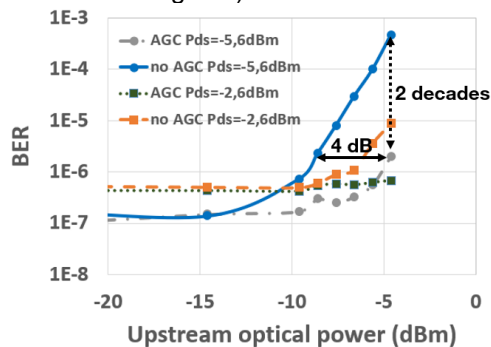
Fig. 6: BER versus US optical power for a DS power of -5.6 dBm (circle) and -2.6 dBm (square) at the input of the SOA with and without AGC.
