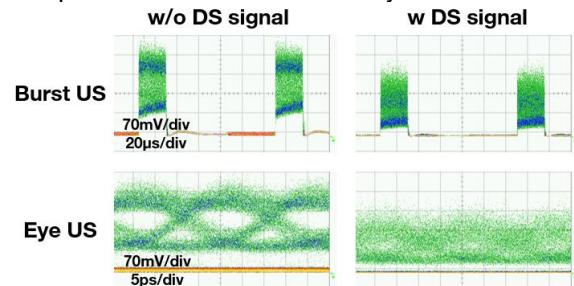
Fig. 7: US burst and eye diagram without and with DS signal.
