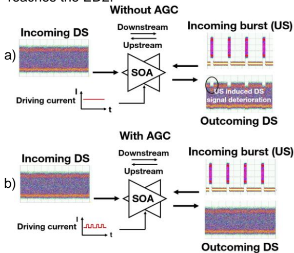
Fig. 3: Behavior of SOA in bidirectional amplification without (a) and with (b) AGC.
