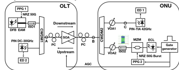
Fig. 1: Experimental setup
