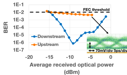
Fig. 4: BER versus average received optical power for DS (blue circle) and US (orange circle).
