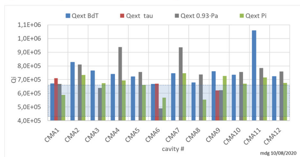
Figure 3: Qext estimation by different methods. Bdt and tau: Eacc exponential decay respectively at 1 MV/m, (performed during the test bench commissioning of each cavity) and at 6.5 MV/m performed at GANIL after installation and cool-down), 0.93-Pa and Pi: RF power indicated by the amplifier (corrected by a factor of 7% loss in the circulator and transmission lines) and by the directional coupler at the cavity entrance.
