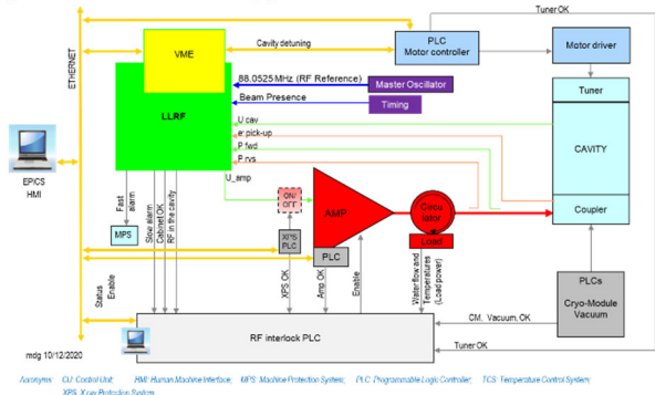
Figure 1: SC cavity RF system block diagram.
