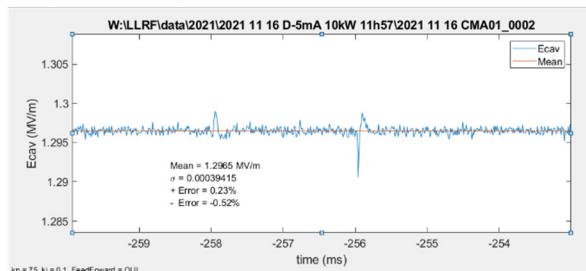
Figure 6: residual field perturbation on cavity A1 with a 5 mA deuteron beam, strong FB and FF. The vertical plot scale is \pm 1\% of the mean value
