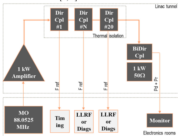
Figure 4: MO and reference distribution bloc diagram.
