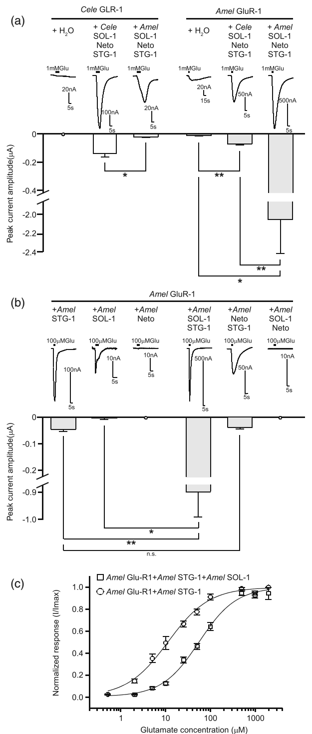
FIGURE 3 Functional reconstitution of A. mellifera GluR-1 in X. laevis oocytes. (a) and (b) top, representative current traces recorded in X. laevis oocytes that express C. elegans GLR-1 or A. mellifera GluR-1 without (+H 2 O) or with the indicated chaperone proteins. Bottom, mean current amplitude for the different protein combinations. Bars represent the mean ± SEM of n = 6–70 oocytes. Values are given in Table 1. * p < 0.01, ** p < 0.001. The line above each trace illustrates the duration of agonist incubation. (c) Concentration–response plots for glutamate-induced currents for Amel GluR-1 + Amel STG-1 with or without Amel SOL-1 fitted with the Hill equation. The data are the means ± SEM of n = 15–18 oocytes. Glutamate EC 50 = 14 ± 3 and 61 ± 7 μM and nHill = 1.0 ± 0.1 and 1.1 ± 0.1 without and with Amel SOL-1, respectively
