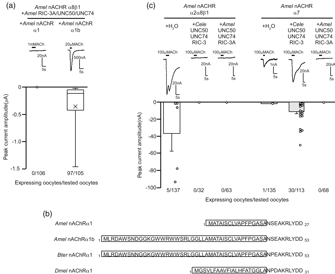
FIGURE 5 Reconstitution of honeybee nAChRs containing the \alpha 1 and \alpha 1b variants. (a) Top, representative current traces recorded in X. laevis oocytes that express either nAChR \alpha 1 or \alpha 1b with the indicated subunits and chaperone proteins. Bottom, box plots of current amplitudes for the two protein combinations. The cross symbol indicates the mean value of n = 97 oocytes from N = 4 frogs. (b) Amino acid sequences of the N terminus of A. mellifera nAChR \alpha 1 (AJE70259) and \alpha 1b (XP_026298411), B. terrestris \alpha 1 (XP_03397561) and D. melanogaster \alpha 1 (NP_524481). The identified signal peptides are boxed. (c) Top, representative current traces recorded in X. laevis oocytes that express the \alpha 2\alpha 8\beta 1 or \alpha 7 honeybee subunits without (+H 2 O) or with the indicated C. elegans or A. mellifera chaperone proteins. Bottom, mean current amplitude for the different protein combinations. Bars represent the means \pm SEM of n = 5 –30 oocytes from N \geq 3 frogs. The line above each trace illustrates the duration of agonist incubation
