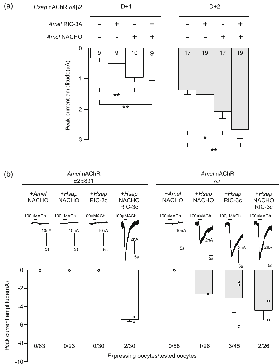
FIGURE 6 Functional reconstitution of honeybee nAChRs with NACHO. (a) Mean current amplitudes recorded at day (D) D + 1 or D + 2 after injection in X. laevis oocytes that express the different protein combinations. Bars represent the means \pm SEM of the indicated number of oocytes from the same batch. The values at D + 1 and D + 2 were as follows: -330 \pm 112 nA and -1375 \pm 143 nA ( \alpha 4\beta 2 without chaperone proteins); -502 \pm 190 nA and -1521 \pm 298 nA ( \alpha 4\beta 2 with A. mellifera RIC-3A); -955 \pm 166 nA and -2075 \pm 229 nA ( \alpha 4\beta 2 with A. mellifera NACHO); and -909 \pm 161 nA and -2665 \pm 288 nA ( \alpha 4\beta 2 with A. mellifera RIC-3A and NACHO), respectively. * p < 0.01 , ** p < 0.001 . (b) Top, representative current traces recorded in oocytes that express the indicated protein combinations. Bottom, mean current amplitudes recorded from n = 2-3 oocytes that express the indicated protein combinations. The mean values are reported in Table 2. The line above each trace illustrates the duration of agonist incubation.
