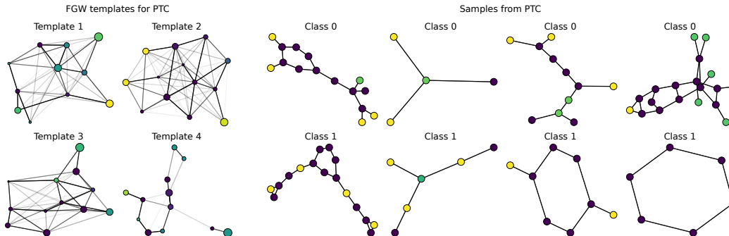
Figure 11: Illustration of the templates learned on PTC with K = 4 and L = 0 (on the left side), and some samples from this dataset (on the right side). The graph structures are represented using the entries of \bar{C}_k (resp. C_i ) as repulsive strength and the corresponding edges are colored in shades of grey (black being the maximum). The node colors are computed based on their features \bar{F}_k (resp. F_i ). The nodes size are made proportional to the weights \bar{h}_k (resp. h_i ).
