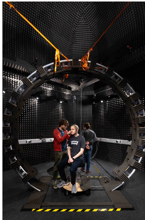
Fig. 1. HRTF measurement setup at Imperial College London (axdesign.co.uk)
